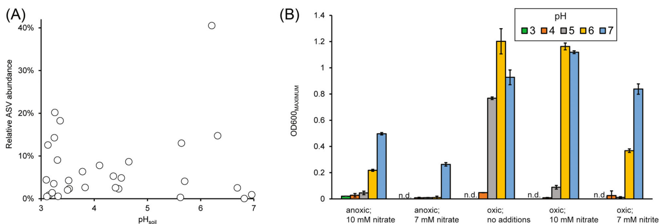
FIGURE 4 Correlation of CPTF-matching ASV range with pH-dependent growth of strain CPTF. (A) The relative abundance of the CPTF-matching ASV is plotted on the vertical axis against the pH of the associated sediment sample. (B) Bars represent the maximum OD_{600} of strain CPTF at varying pH values under different growth conditions in batch culture. The figure legend indicates the pH of the culture: pH 3 (green), 4 (orange), 5 (grey), 6 (yellow), 7 (blue). Glucose (20 mM) was added as the carbon source for all experiments. pH 3 data were only collected for the anoxic nitrate-respiring cultures. Graphed data are the average of three biological replicates and error bars represent \pm SD.
