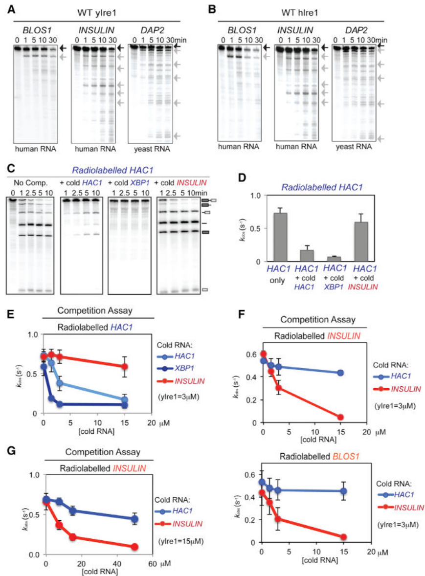
Figure 1. In Vitro Cleavage of RIDD Substrate RNA Is Distinct from XBP1/HAC1 Cleavage (A and B) In vitro cleavage of RIDD. In vitro transcribed radiolabeled mammalian ( BLOS1 , INSULIN ) and yeast ( DAP2 ) RNA substrates (0.5 nM) were incubated with ADP (2 mM) and 1 \mu M recombinant WT yIre1 (A) or WT hIre1 (B) for up to 30 min. Black arrow, full-length RNA; gray arrow, cleaved RNA fragments. (C and D) Using single-turnover conditions (Figure S1F), HAC1 RNA cleavage reactions were competed by excess unlabeled (cold) HAC1 or XBP1 RNA (15 \mu M) but not with RIDD RNA (15 \mu M). Reactions were performed with 2 mM ADP for up to 10 min. (C) k_{obs} calculated from these reactions are shown in (D). Error bars of all the experiments in this figure represent at least three independent repeats. (E) HAC1 RNA cleavage reactions with different concentrations of various competitor RNAs (representative reactions shown Figures S1G and S1H).
