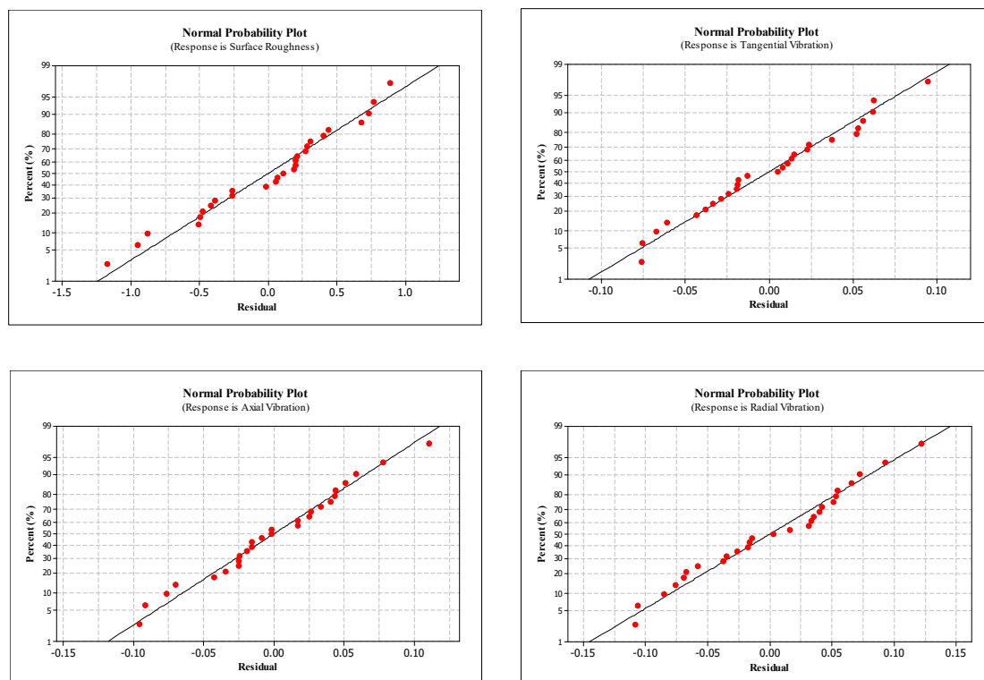
Figure 5. Normal probability plots for surface roughness and vibration.
