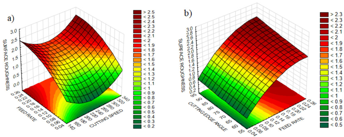
Figure 4. The effect of parameters on surface roughness (a) Combination of feed rate and cutting speed (b) Combination of cutting edge angle and feed rate.
