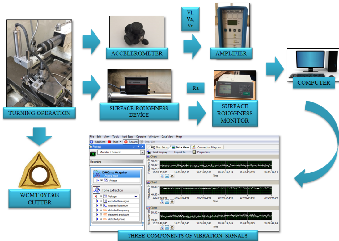
Figure 1. Experimental setup.
