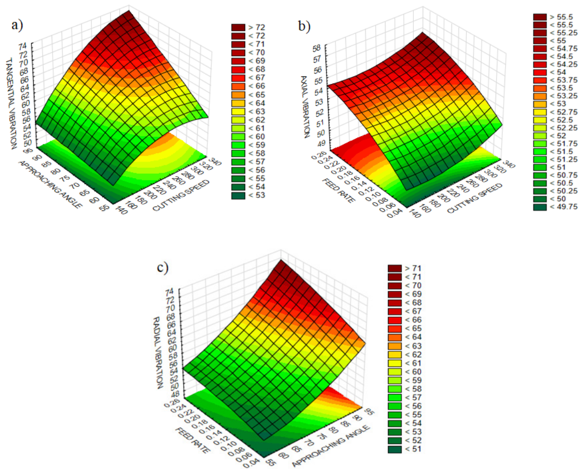
Figure 3. The influential parameters on 3 components of vibration (a) The effect of cutting edge angle and cutting speed on tangential vibration, (b) The effect of feed rate and cutting speed on axial vibration, (c) The effect of cutting edge angle and feed rate on radial vibration.
