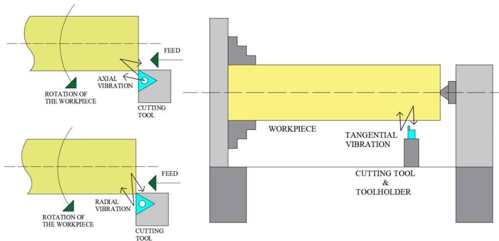
Figure 2. Vibration components occurring on the machine tool.
