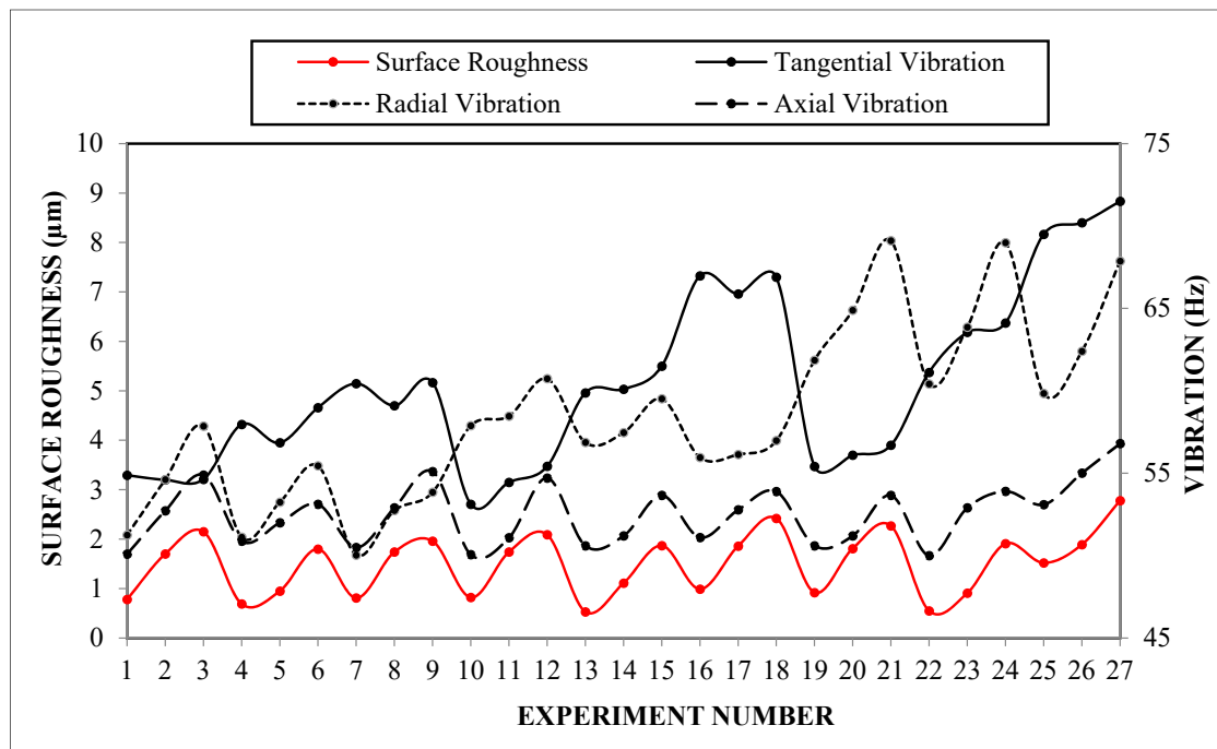
Figure 6. Interaction between surface roughness and vibration components.
