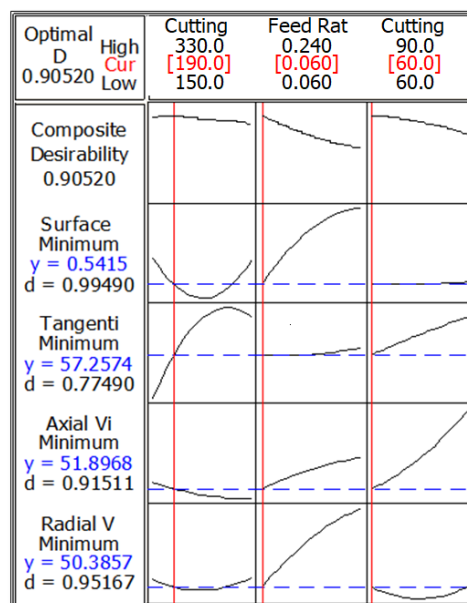
Figure 7. Optimum cutting conditions for minimum surface roughness and vibration.
