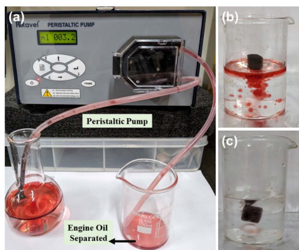
Fig. 9 The separation of oil from water using the g-C 3 N 4 /Bi 2 S 3 foam by: (a) continuous separation facilitated by a peristaltic pump, and (b and c) continuous stirring of oil in water.
