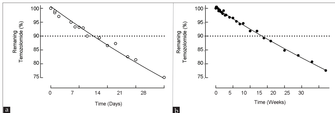
Figure 2: Stability of temozolomide in solutions aimed for oral use prepared from Temodal™ powder for infusion solution. (a) Initial concentration: 2.5 mg/mL; Temperature: 22°C. The solid line is given by nonlinear regression analysis (one-phase decay; weighted 1/y; r^2=0.9990 ; total n=27 ). (b) Initial concentration: 1.25 mg/mL; Temperature 5°C. The solid line is given by nonlinear regression analysis (one-phase decay; weighted 1/y; r^2=0.9955 ; total n=26 )
