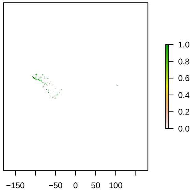
S4Dryas_iulia
