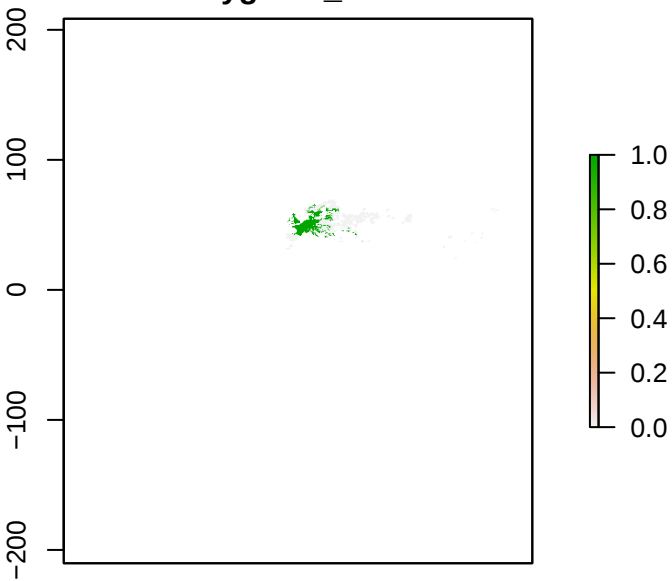
S1Polygonia_c.album
