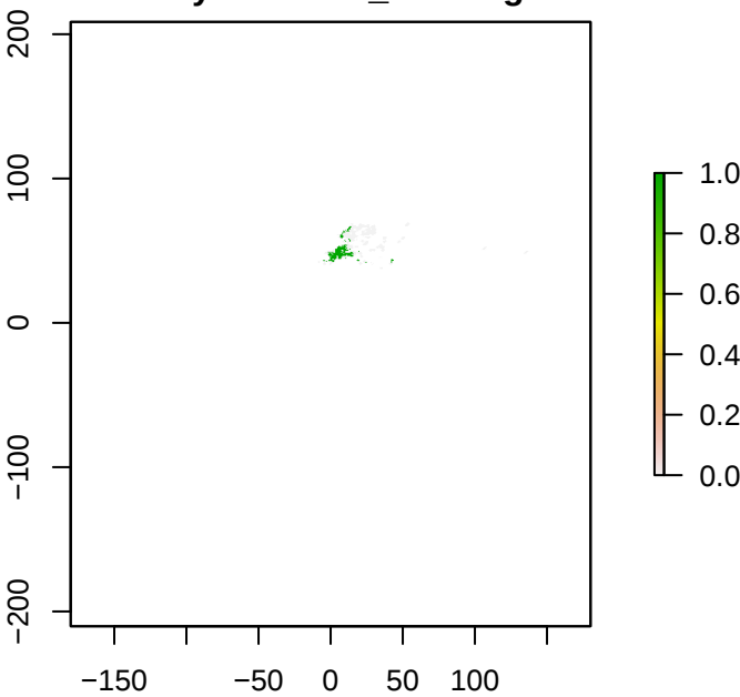
S3Polyommatus_semiargus
