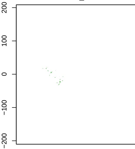
S1Eueides_isabella
