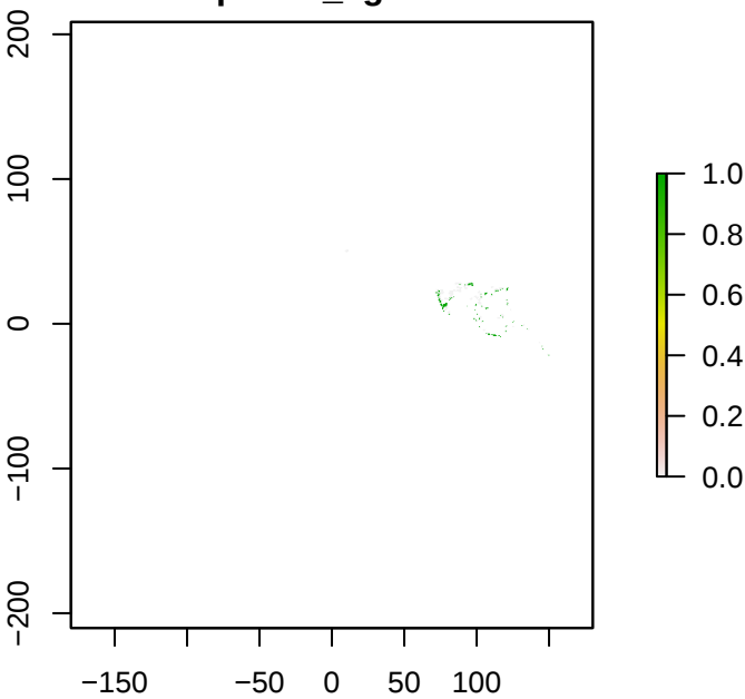
S3Graphium_agamemnon
