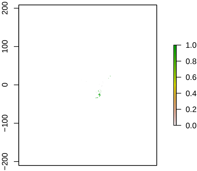
S1Anthene_amarah
