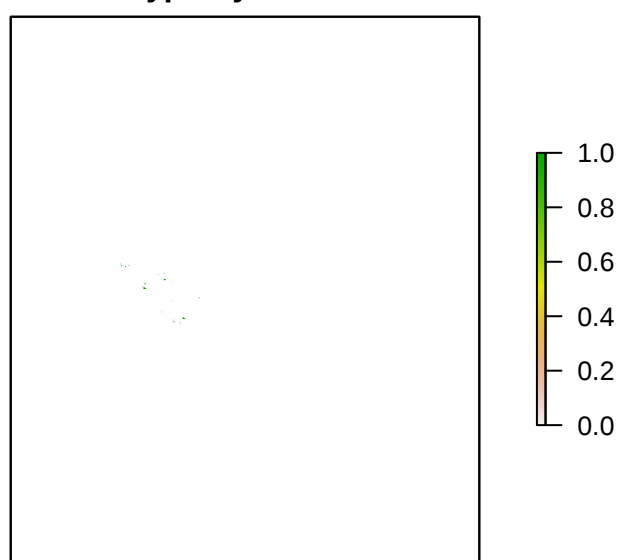
S2Hypothyris_euclea
