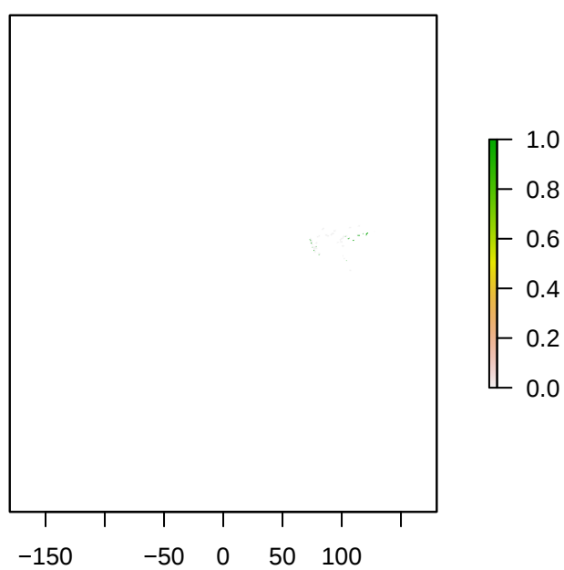
S4Jamides_bochus
