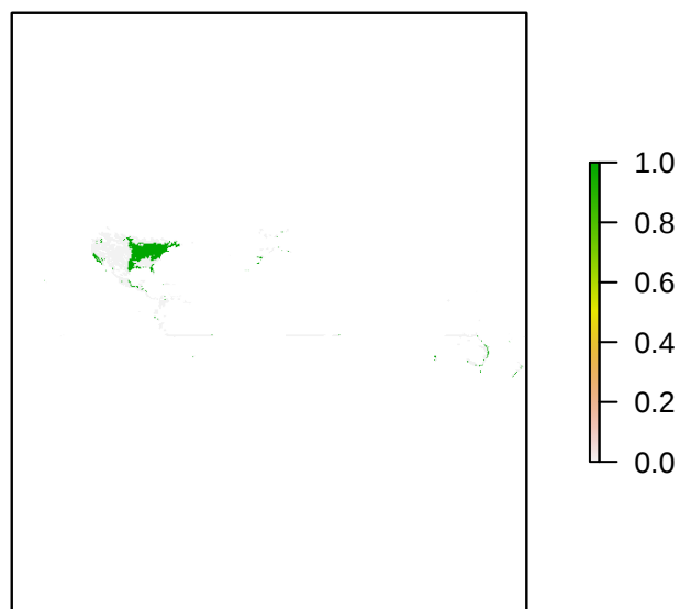
S2Danaus_plexippus
