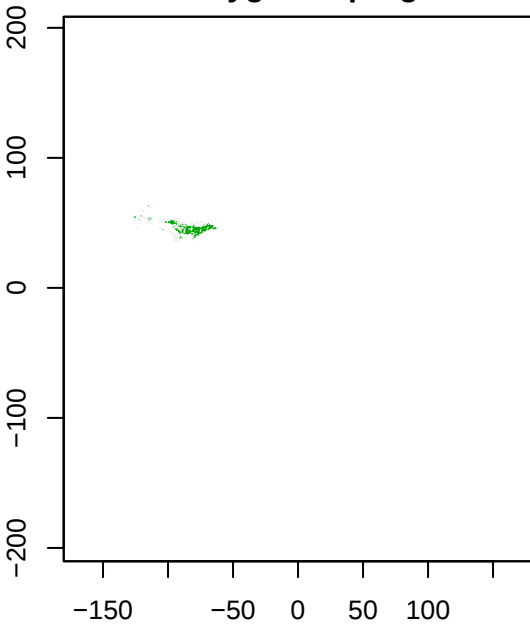
S3Polygonia_progne
