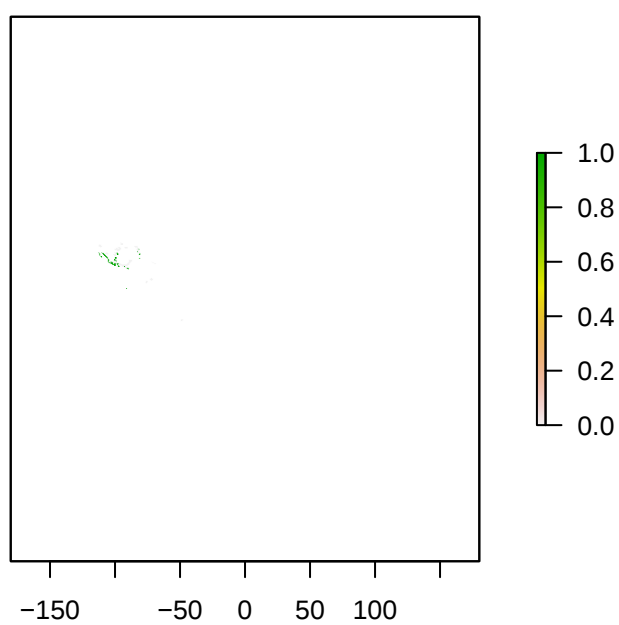
S4Urbanus_dorantes
