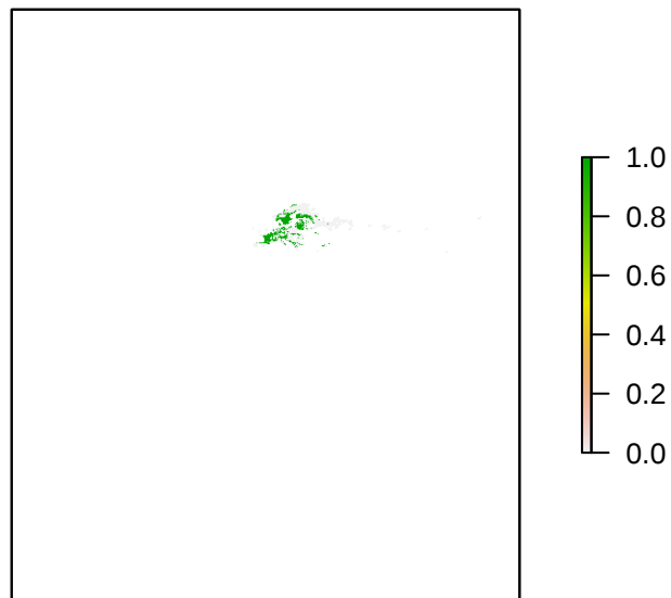
S2Melitaea_athalia
