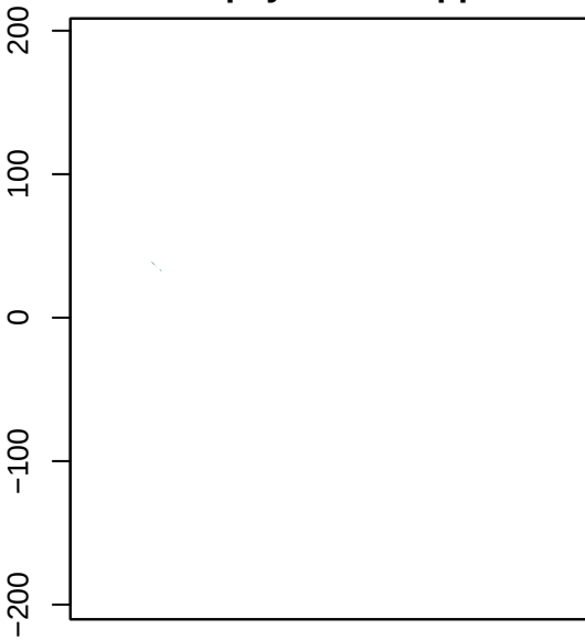
S1Speyeria_callippe
