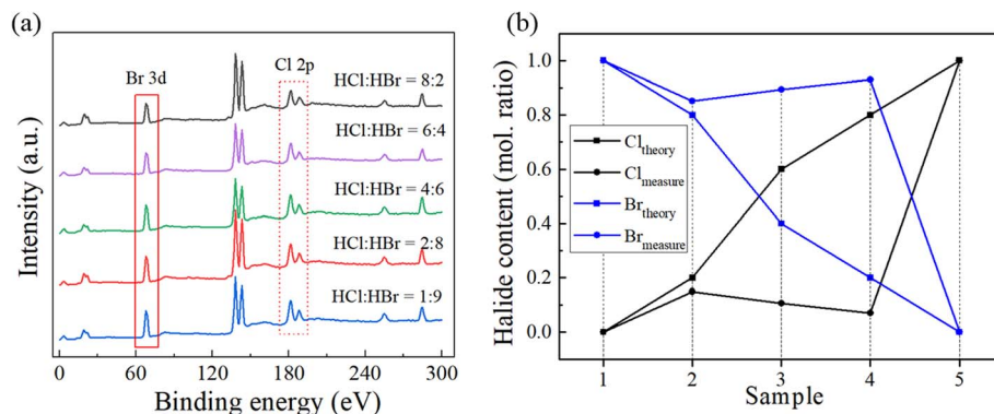
Fig. 4 (a) XPS survey of (\text{BA})_2\text{Pb}(\text{Cl}-\text{Br})_4 fabricated in mixed HX solutions. (b) Comparison of the measured and theoretical contents of Cl and Br in the (\text{BA})_2\text{Pb}(\text{Cl}-\text{Br})_4 single crystals.
