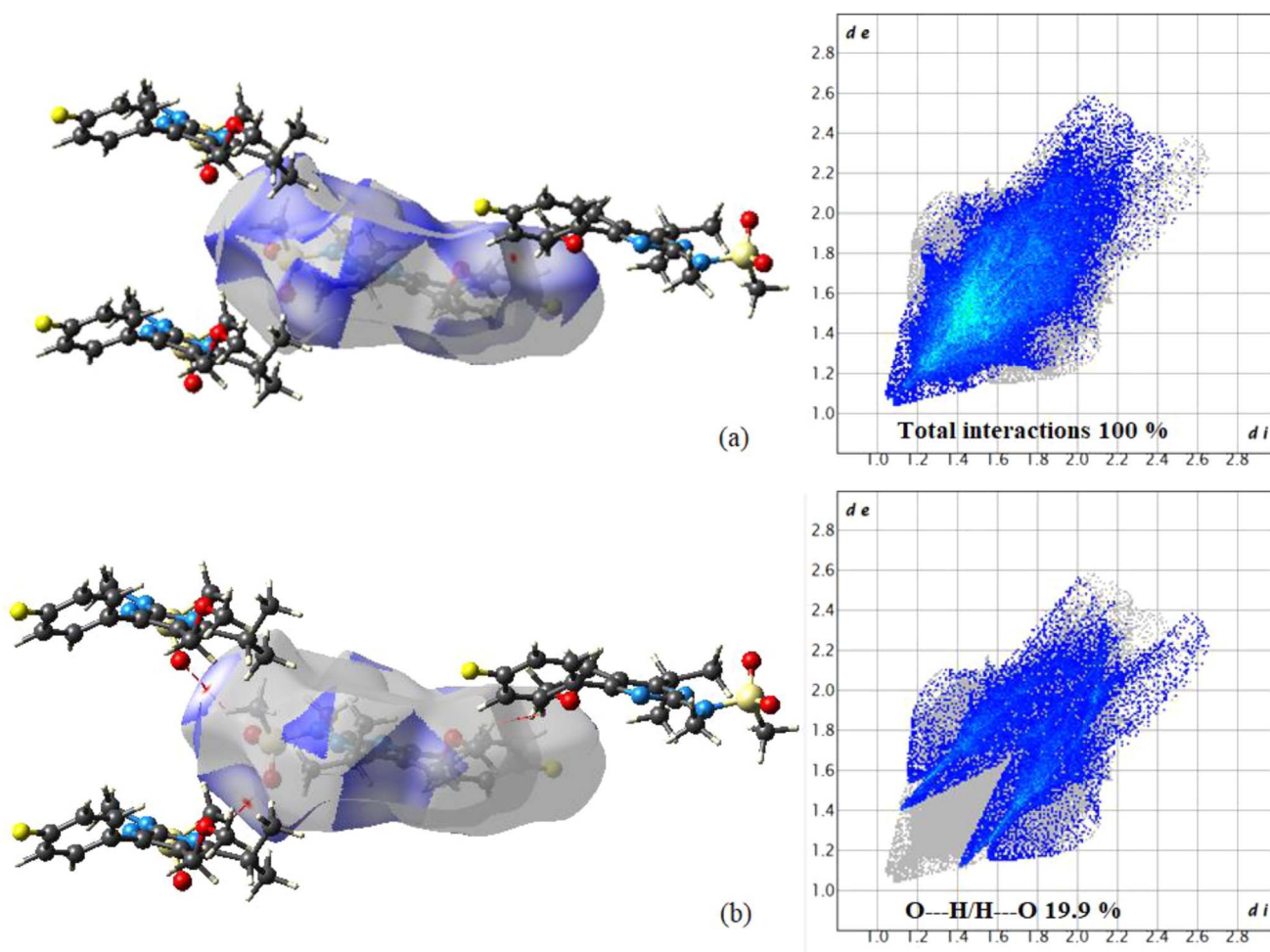
Fig. 4 Hirshfeld surface analysis of PMMS: (a) Hirshfeld surfaces mapped with d_{norm} showing interactions with neighboring molecules; (b) O...H/H...O contacts on the d_{norm} surface with the fingerprint plot.
