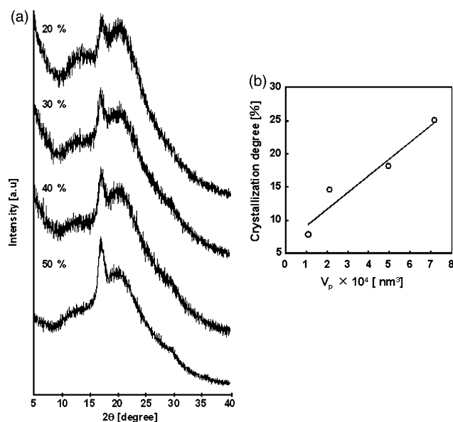
Fig. 7. (a) XRD patterns of poly{styrene- co -acrylonitrile- co -poly(ethylene glycol) monomethoxymonomethacrylate} prepared with water compositions of 20 ( V_p = 7.19 \times 10^4 \text{ nm}^3 ), 30 ( V_p = 4.98 \times 10^4 \text{ nm}^3 ), 40 ( V_p = 2.15 \times 10^4 \text{ nm}^3 ), and 50% ( V_p = 1.12 \times 10^4 \text{ nm}^3 ). (b) Relation ship between crystalline degree AN units and projection volume, V_p .
