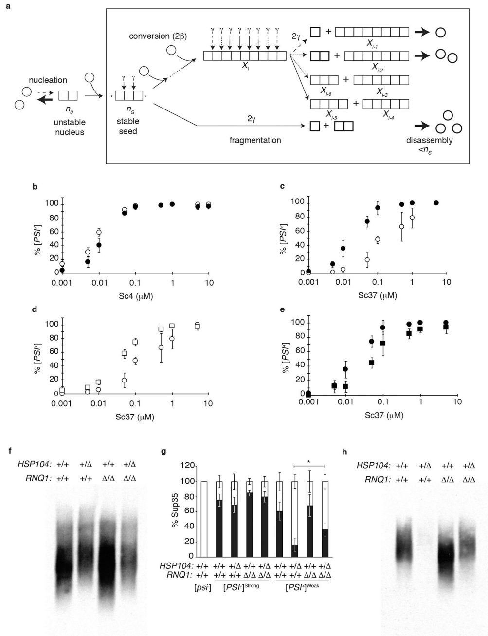
Fig 1. [PIN^+] and deletion of Hsp104 combine to impact appearance and propagation of [PSI^+]^{Weak} . a. Native monomer (circle) spontaneously and rarely (dashed arrow) associates to form a nucleus of size n_0 , the rate-limiting step for amyloid formation. The nucleus is thermodynamically unstable (solid, heavy back arrow), and subsequent addition of monomers through favorable associations ultimately creates a stable seed of minimum size n_s . The seed can grow at a rate that is double the single-site conversion rate ( 2\beta ) because monomers can add to either end of the aggregate (*). The seed or any larger aggregate may be fragmented at any monomer junction (down arrows) at a single-site fragmentation rate
