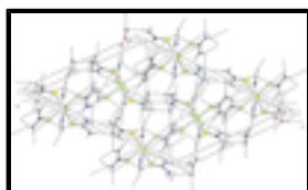
Fig. 2. Partial view of the intra and intermolecular N—H...S and N—H...O hydrogen bonds in the crystal structure of (I), forming a three-dimensional network.
