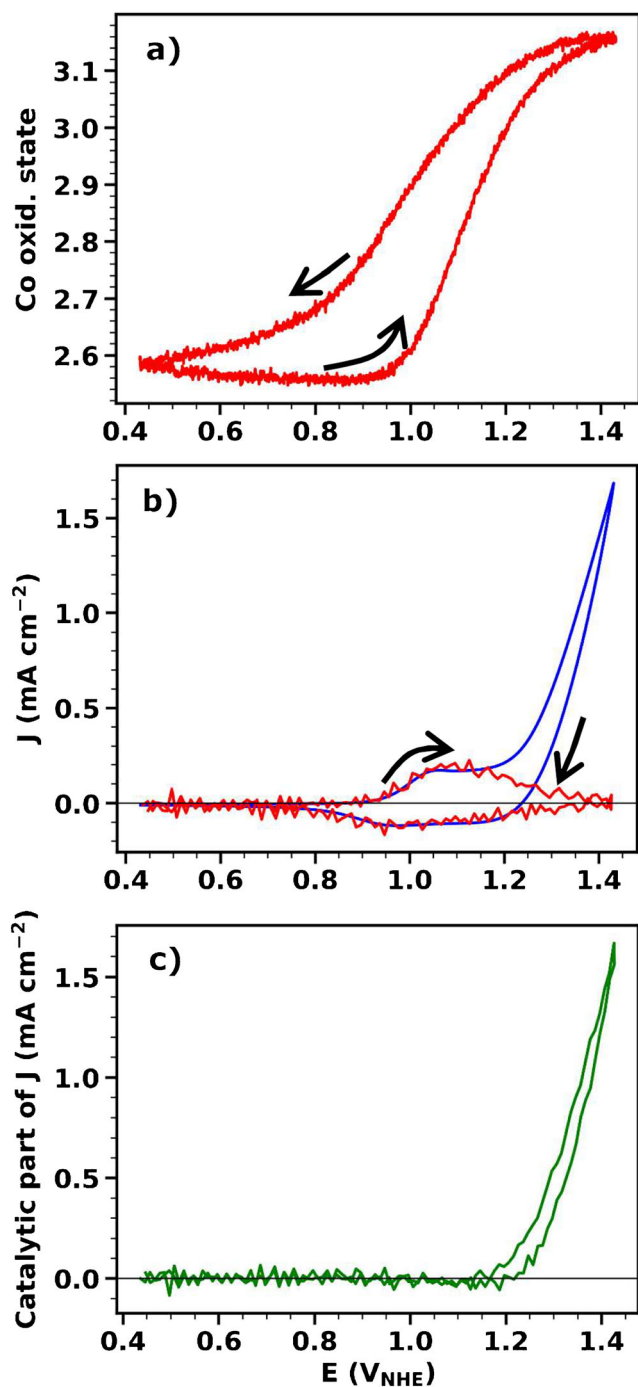
Fig. 6 Cyclic voltammetry experiment (scan rate 10 \text{ mV s}^{-1} ) for a CoCat sample (thickness 90 \text{ nm} , corresponding to 12.5 \text{ mC cm}^{-2} ) operated in 0.1 \text{ M KPi} electrolyte at \text{pH } 7 . Data averaged from 14 CVs are shown. a Average oxidation state of the Co ions. For excitation at 7722 \text{ eV} (center of Co absorption K-edge), the continuously recorded X-ray fluorescence was converted to an average Co oxidation state following the procedure described in Fig. 1. b Current density (blue line) and redox current density (i.e., component of the current responsible for oxidation state changes, red line), obtained from the derivative of the fluorescence signal by means of Eq. 2. The dissolution factor (see Eq. 3) was set to 0.7 , resulting in excellent agreement between the redox current and the measured electric current in the redox-wave CV region. c Catalytic current density calculated as the difference between the total measured current density and the redox current density calculated from the derivative of the oxidation-state signal by means of Eq. 2. The black arrows indicate the scan direction
