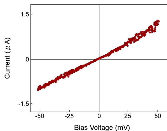
Figure 2. Current–voltage characteristics of the SNPJ presented in Fig. 1(a). The resistance near 0 V is 4.2 kΩ.
