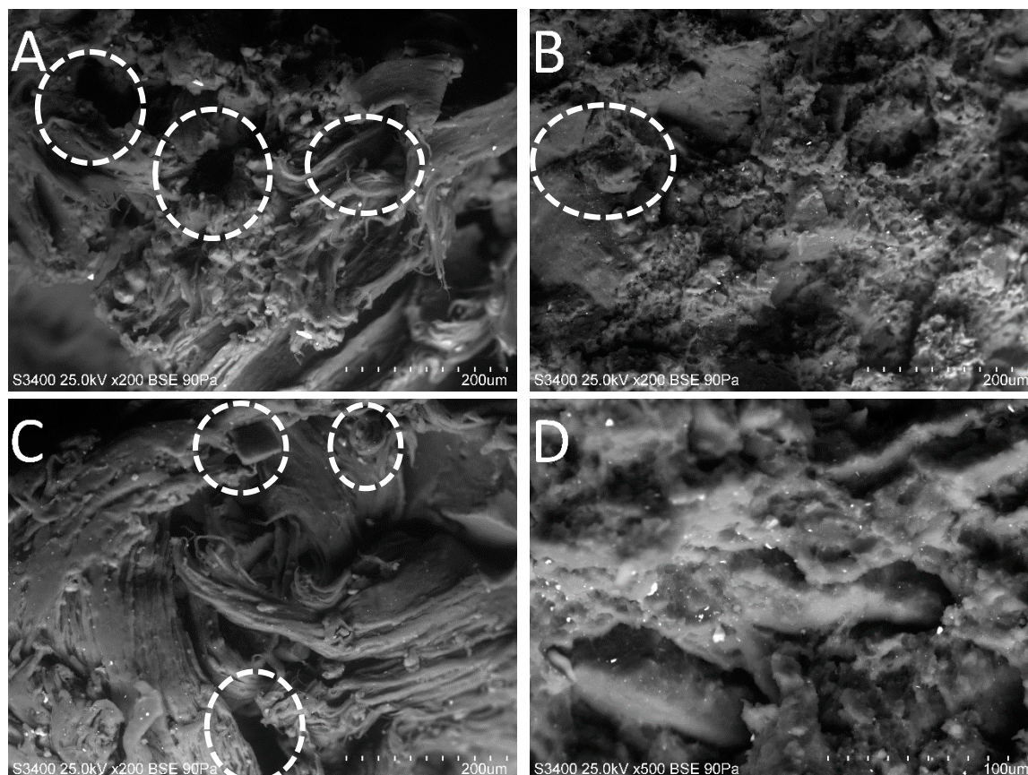
Figure 10. SEM images of surface after tensile test: (A)—RR:PCL(6800) 50:50; (B)—RR:PCL(6800) 90:10; (C)—RR:PCL(FB100) 50:50; (D)—RR:PCL(FB100) 90:10.
