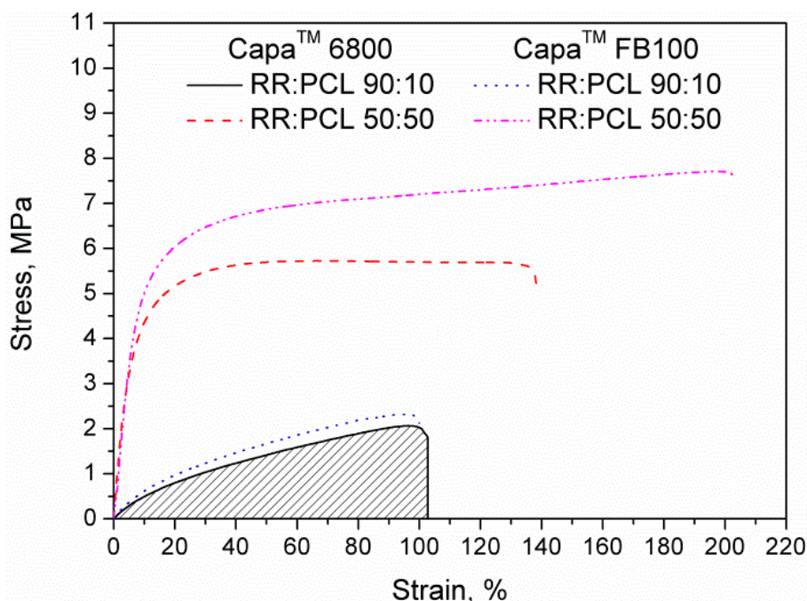
Figure 2. Stress–strain curves of RR/PCL blends.
