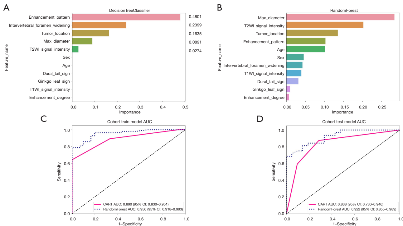
Figure 5 The importance of the variables in the CART and RF models, respectively. (A) CART model; (B) RF model. The ROC curves of the CART and RF models in the training and test groups, respectively. (C) Training group; (D) test group. AUC, area under the curve; CART, classification and regression tree; RF, random forest; ROC, receiver operating characteristic.
