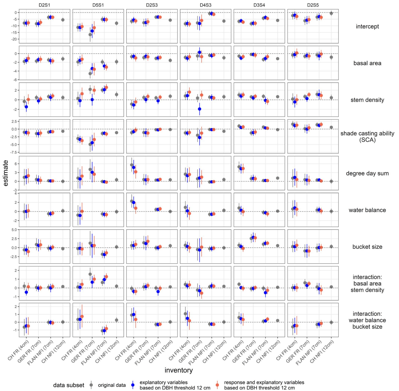
FIGURE 4 Comparison of models with modified inventory. Shown are expected effect sizes (dots) with 95% credible intervals (vertical lines). Model fits based on the original data sets without modified DBH are shown in gray. Model fits based on data where the DBH threshold for explanatory variables was artificially increased to 12 cm are shown in blue. Model fits based on data sets where both explanatory variables and abundance of tree recruitment were calculated with a DBH threshold of 12 cm are shown in red. Note that the gray bars correspond to the same values shown in the trait group-specific values shown in Figure 3. For a description of the trait groups (D2S1, D5S1, D2S3, D4S3, D3S4, D2S5) see Figure 2, Table A4, and Figure A5
