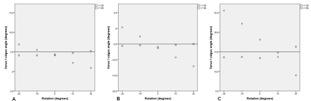
Fig 5. EOS 2D/3D measurements and measurement errors of varus/valgus angle for different combinations of preset varus/valgus angle and flexion angle and rotation.
