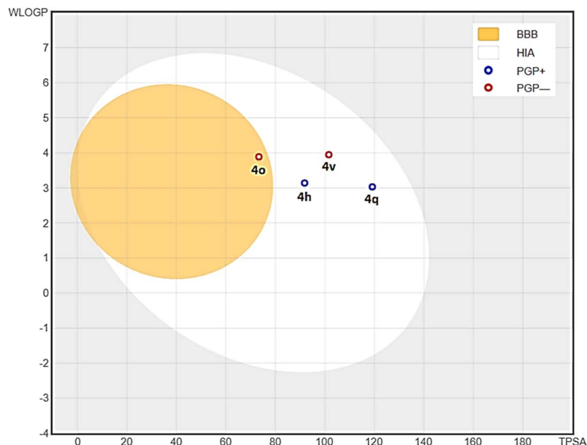
Fig. 4 BOILED-Egg model of 2,4-dimethoxy-THPQs 4h, 4o, 4q and 4v.
