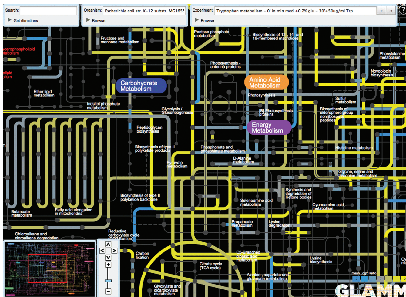
Figure 3. Experimental data visualization. Overlay of expression data collected during a metabolism experiment on E. coli K12 substr. MG1655. The reactions corresponding to upregulated genes are shown in yellow, reactions corresponding to downregulated genes are shown in blue.
