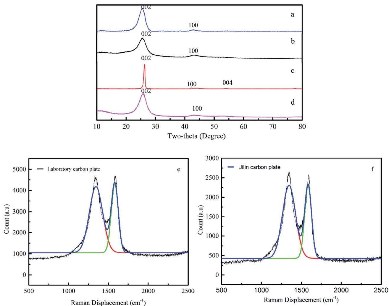
Fig. 7 XRD patterns of (a) laboratory and (b) Jilin carbon plates, (c) graphite sample and (d) petroleum coke raw material. Raman spectra of (e) laboratory and (f) Jilin carbon plates.
