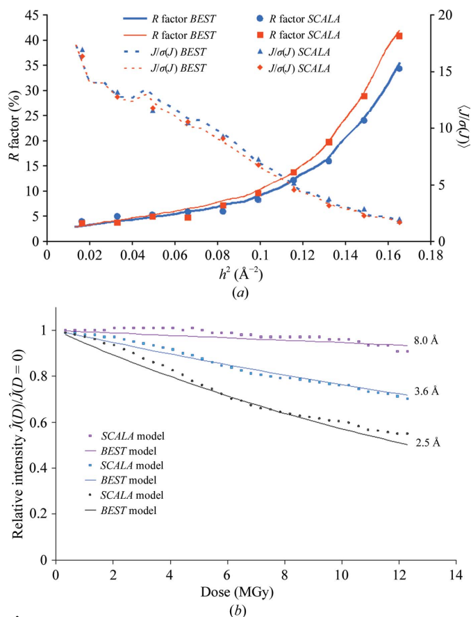
Figure 4 Test-data collection for the P19–siRNA-1 crystal. (a) Predicted and experimental R_{\text{merge}} (solid line) and \hat{J}/\hat{\sigma} (dashed line) versus resolution for P19–siRNA-1A (blue) and P19–siRNA-1B (red). (b) Predicted and experimental relative diffraction intensities, \hat{J}(D)/\hat{J}(D=0) , versus the dose and resolution for P19–siRNA-1B.
