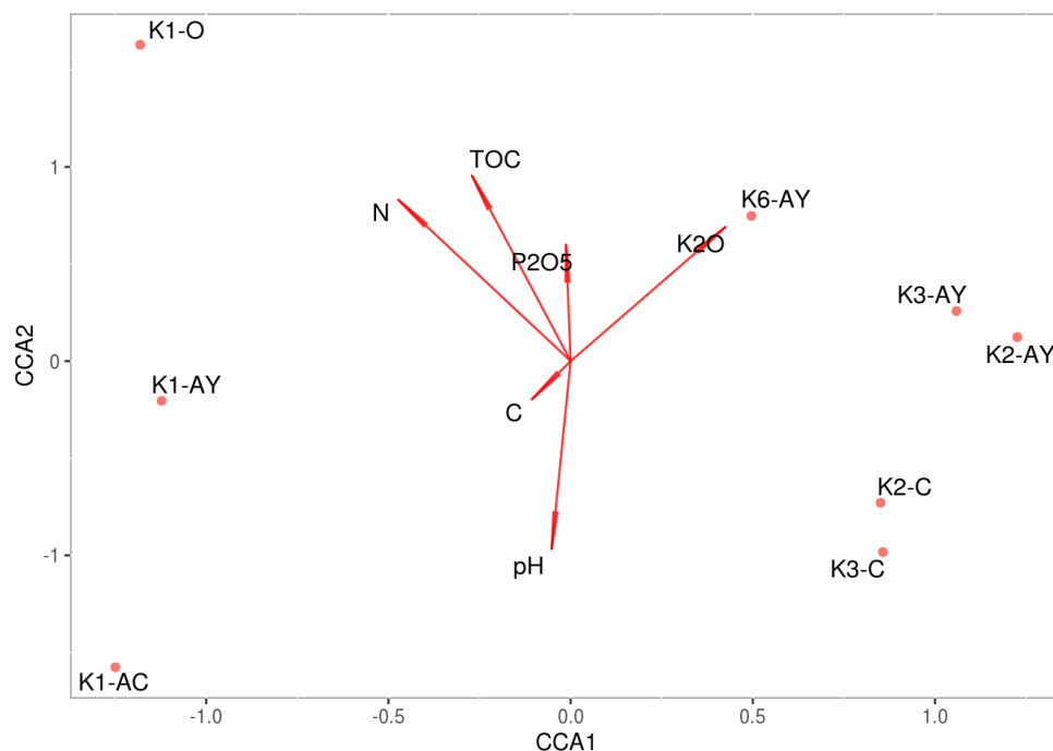
Figure 6 CCA. Direction of the vectors shows the degree of covariation between factors.
