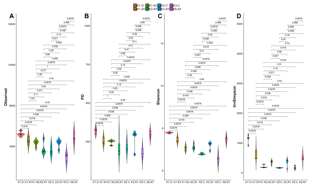
Figure 4 Alpha diversity indexes for each soil horizon. (A) Observed, (B) PD, (C) Shannon, (D) inverted Simpson. Data presented by violin and box plots, which show the kernel probability density of the data at different sample values. P -values are given above plots.
