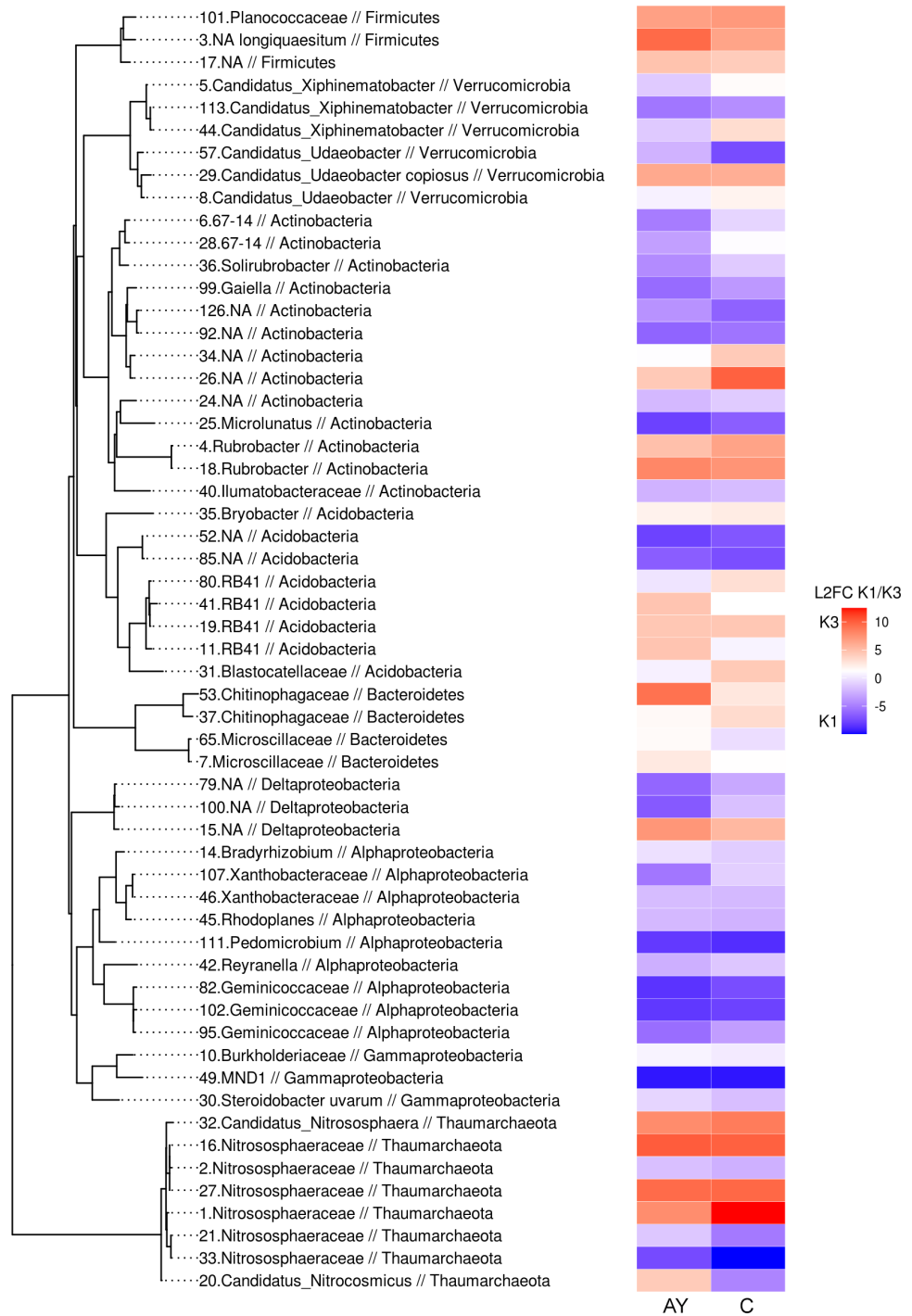
Figure 7 Phylogenetic tree with phylotypes, which abundance shifts significantly ( p_{adj} < 0.05 ) between K1 and K3 sites. Shifts are presented as log 2 foldchange values. The left column shows shifts in the AY horizon, right column, the AC/C horizon. Red indicates an increase in K3, blue, in K1.
