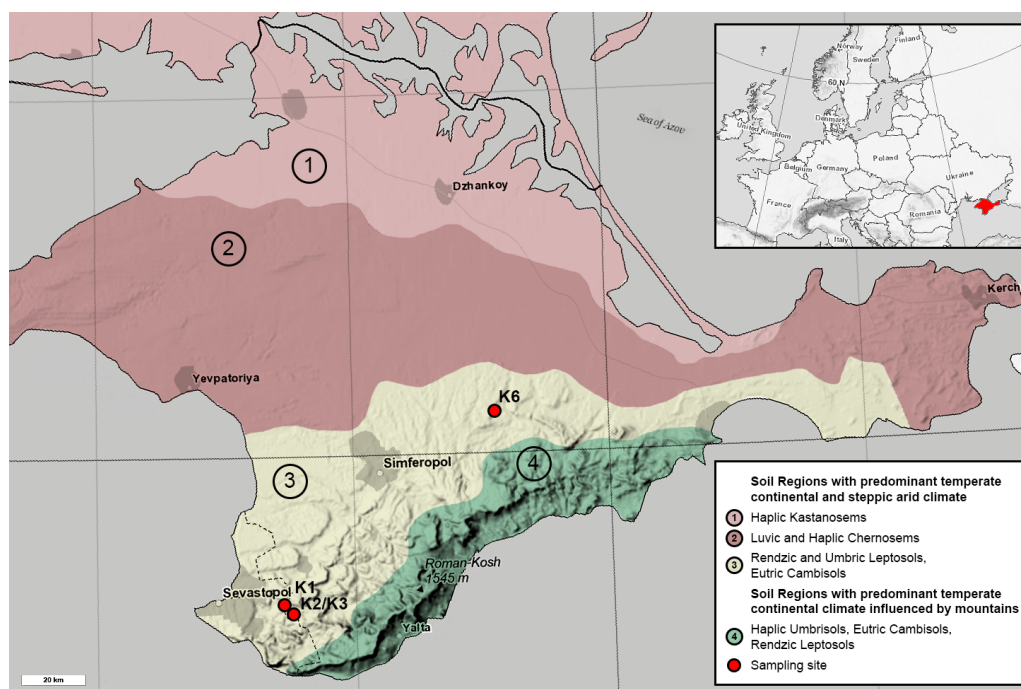
Figure 1 Map of the Crimean Peninsula and the location of sampling sites. Modified after Soil Regions Map of the European Union and Adjacent Countries (BGR, 2005). Colour and numbers 1-4 mark different soil types. Sampling sites are marked with red circles.
