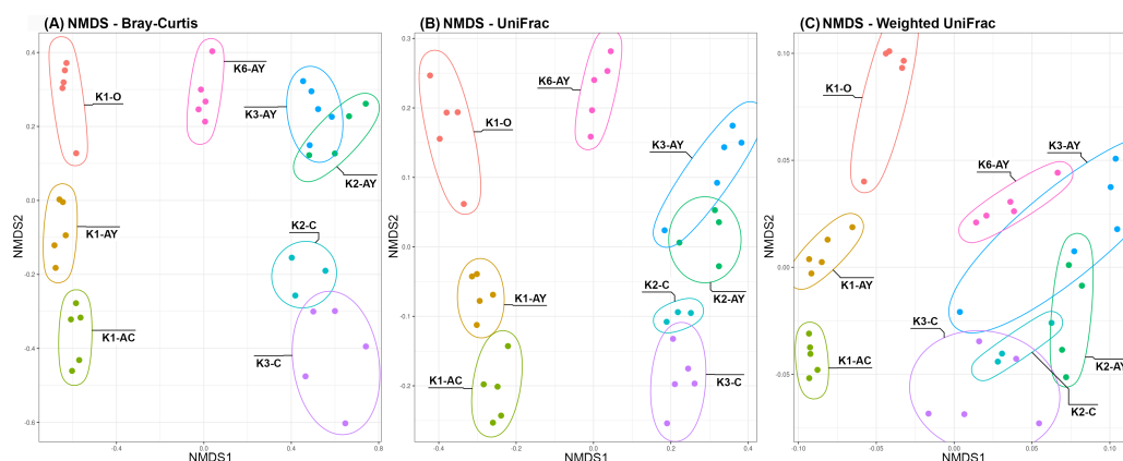
Figure 5 NMDS plots of Beta diversity. (A) Bray–Curtis distance matrix. (B) UniFrac. (C) weighted UniFrac. Sample repeats are surrounded by ellipses, estimated using the Khachiyan algorithm.
