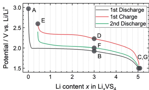
Fig. 2 Charge–discharge profile of the \text{Li}/\text{a-}\text{VS}_4 cell between 1.5 and 2.6 V. Sampling points are marked on the figure.
