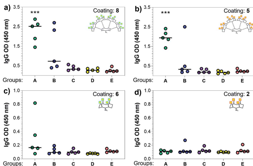
Fig. 4 Analysis of total IgG antibodies elicited against the synthetic glycosylated scaffolds. Microtiter plates were coated with the four different glycosylated scaffolds lacking the OVA epitopes: (a) 8, (b) 5, (c) 6, and (d) 2 (see Scheme 1); and the antisera from mice A to E were probed. Statistical significance compared to no-adjuvant control group (Group E) was assessed using two-tailed unpaired Student's t -test: *** p < 0.001.
