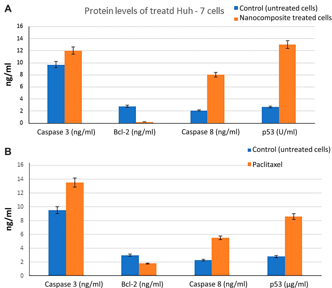
Figure 7 (A). Effect of curcumin chitosan nanocomposite treated Huh7 on protein levels of Caspase 3, Bcl-2, caspase 8, and p53, (B). Effect of paclitaxel treatment on the expression levels of the same proteins. Error bars represent standard deviation.
