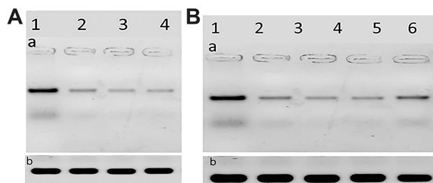
Figure 8 (A). The scanned densitometry Western blot of viral replication in Huh7 (a) versus \beta -actin (b). Lane 1: protein levels of infected cells treated, Lane 2: infected cells treated with curcumin, Lane 3: infected cells treated with chitosan nanoparticles, Lane 4: infected cells treated with curcumin chitosan nanocomposite, (B). The scanned densitometry Western blot of viral entry (a) versus \beta -actin (b) protein levels in positive Lane 1: untreated infected cells, Lane 2: cells treated with CsNPs, Lane 3: cells treated with nanocomposite, Lane 4: cells treated with nanocomposite, Lane 5: cells treated with curcumin, Lane 6: cells treated with sovaldi. HCV core protein at size of 22 KD.
