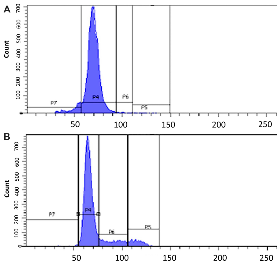
Figure 6 (A). Cell cycle analysis of untreated Huh7 cells, (B). Cell cycle analysis post-treatment of Huh7 with IC 50 concentration of nanocomposite, showing preG1 arrest by 6.7% compared to control cells and therefore inhibiting cells from entering S phase and G2/M phase.
