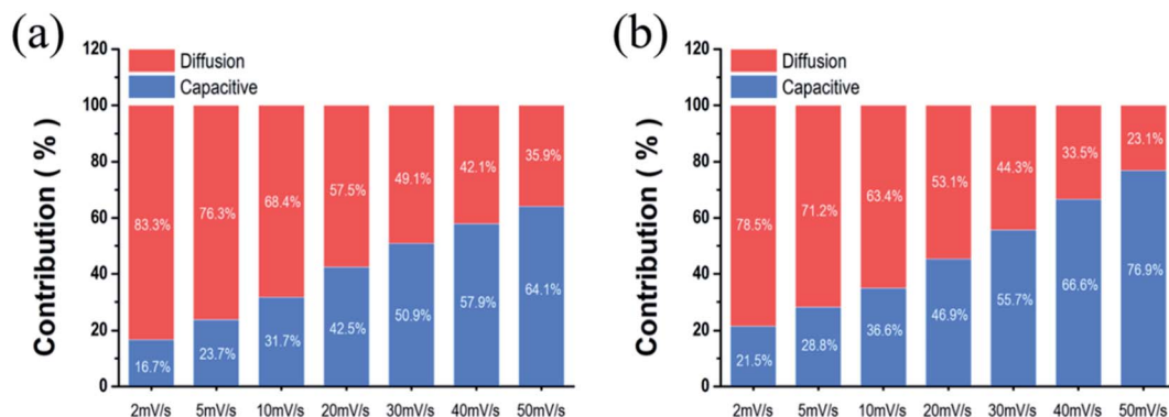
Fig. 6 Comparison of the capacitive contribution and diffusion-controlled contribution to current of (a) NiCo LDH and (b) NiCo LDH-SP (1) .
