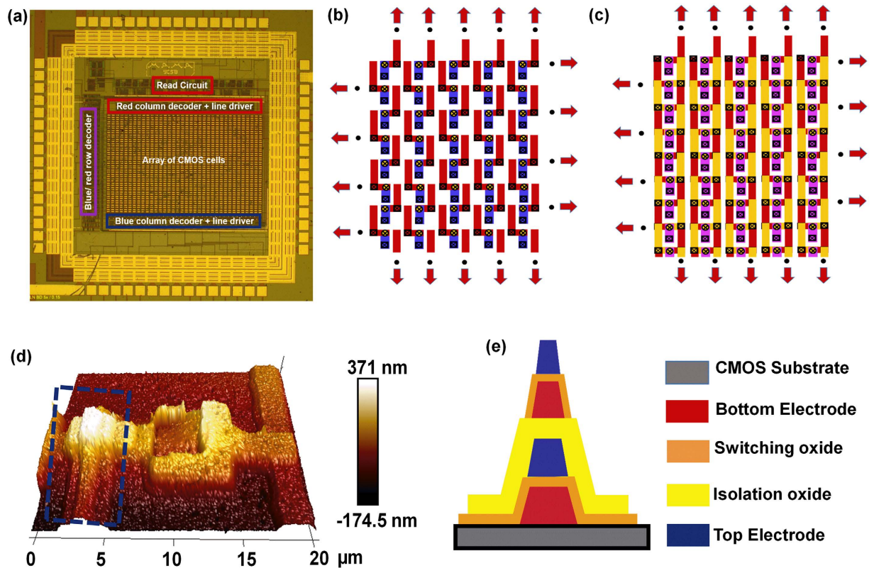
Figure 2. Fabrication of a 3D CMOL crossbar. (a) Optical image of the foundry-processed CMOS chip showing the on-chip decoder, 'Read' and 'Write' circuitry as well as the 24 \times 36 array of CMOS cells. Each 'CMOS cell' houses a pair of pins ('Red' and 'Blue'), (b) structure of the first layer of the 3D crossbar, (c) the final structure of the 3D crossbar with 2 layers (d) AFM image of a section of the 3D crossbar: the highlighted section shows two stacked device layers, (e) Cross-section of the region highlighted in (d).
