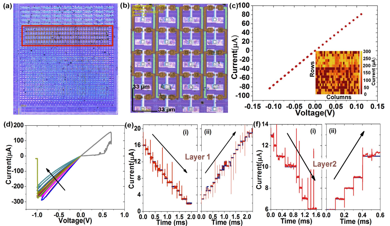
Figure 4. Electrical characteristics. (a) An optical image of the CMOS chip with vertically integrated memristive crossbars: the region highlighted in the red box has the 3D CMOL crossbar structures, (b) A high-resolution optical image of a section of the integrated 3D crossbars. (c) A typical I - V plot measured on a test structure to test the contact resistance between the memristive layer and the underlying CMOS. Inset shows a map of the current measured at all the 24 \times 36 array of 'red pins' showing contact between the integrated devices and the CMOS cells. Current is measured at 0.2\text{ V} for each measurement. (d) An I - V plot showing typical DC switching characteristics of the integrated memristive devices: the device is initially turned on and is gradually reset demonstrating analog switching behavior, (e) pulsed switching characteristic of a device in layer 1 showing gradual reset and set operation: the device is tuned to each desired state using a tuning algorithm (discussed in the supporting info.). The arrow indicates the direction of programming in each case, (f) pulsed switching characteristic of a device in layer 2 showing gradual reset and set operation: the device is tuned to each desired state using the tuning algorithm.
