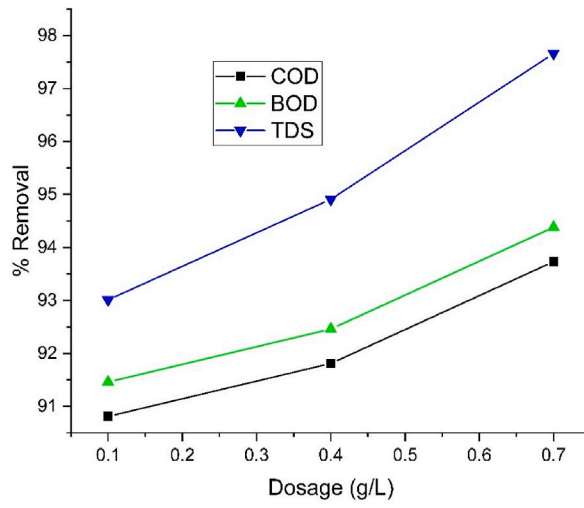
Fig. 6. Effect of dosage on coagulation process.
