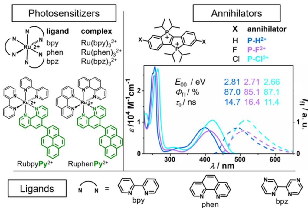
Fig. 3 Left and bottom: Ruthenium complexes and dyads with the respective ligands used as photosensitizers (PS), for more details see ref. 4, 19 and 27. Right: Novel annihilator structure (P-H 2+ ) 47 and derivatives (P-F 2+ , P-Cl 2+ ), their calibrated UV/vis absorption and emission spectra and basic photophysical characteristics in Ar-saturated 50 mM H 2 SO 4 (see ESI† for details).
