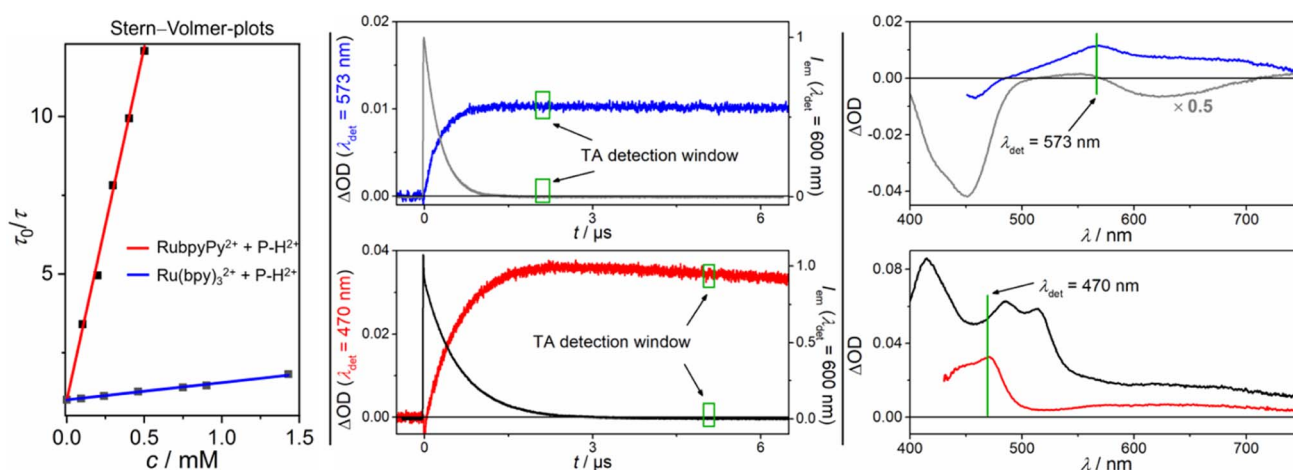
Fig. 4 Left panel: Stern–Volmer plots for the triplet quenching with \text{P-H}^{2+} using {}^3\text{RubpyPy}^{2+} (red fit) and {}^3\text{Ru}(\text{bpy})_3^{2+} (blue fit) as photosensitizers; Central panel: Kinetic sensitizer emission traces (upper for {}^3\text{Ru}(\text{bpy})_3^{2+} in gray, concentration 30 \mu\text{M} , \lambda_{\text{exc}} = 532 nm, 42 mJ and lower for {}^3\text{RubpyPy}^{2+} in black, concentration 31 \mu\text{M} , \lambda_{\text{exc}} = 532 nm, 42 mJ) with \text{P-H}^{2+} (2.0 mM with \text{Ru}(\text{bpy})_3^{2+} , 0.5 mM with \text{RubpyPy}^{2+} ), together with the formation kinetics of the quenching products (blue trace corresponds to the one electron reduced \text{P-H}^+ after ET, red trace corresponds to the {}^3\text{P-H}^{2+} after EnT); Right panel: TA spectra of the triplet excited photosensitizer (upper, gray spectrum {}^3\text{Ru}(\text{bpy})_3^{2+} , and lower, black spectrum {}^3\text{RubpyPy}^{2+} ) and {}^3\text{P-H}^{2+} (red, lower graph) after EnT or \text{P-H}^+ and \text{Ru}(\text{bpy})_3^{3+} (blue, upper graph) after ET. All measurements were carried out in 50 mM \text{H}_2\text{SO}_4 . Further explanations are given in the text and ESI.†
