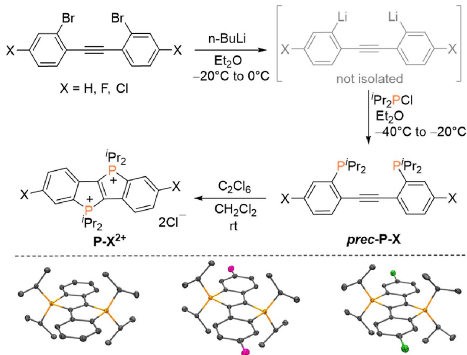
Fig. 2 Top: Synthesis of annihilators P-H 2+ , P-F 2+ and P-Cl 2+ (X = H, Cl, F). Bottom: ORTEP plots of the dications in P-H 2+ , P-F 2+ and P-Cl 2+ (hydrogen atoms, Cl - counter ions and co-crystallized solvents omitted for clarity, see ESI† for details).
