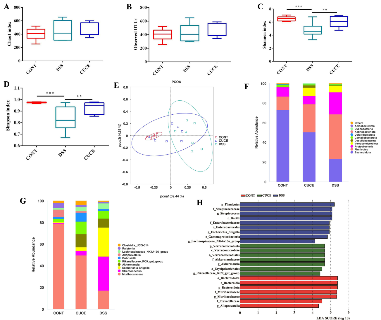
Figure 4 Cucurbitacin E improves microbiota composition in DSS-treated mice. (A) Chao1 index; (B) Observed OTUs; (C) Shannon index; (D) Simpson index; (E) PCOA plot of the microbiota based on a weight UniFrac metric. Relative abundance of predominant bacteria at the phylum (F) and genus (G). (H) Bacterial biomarkers in each treatment group (LDA score value > 4 or < -4). Data are presented as mean ± SEM. **P<0.01, ***P<0.001, n=7.
