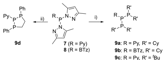
Scheme 4 Synthesis of triphosphanes 9a–c : (i) + 2 eq. R' 2 PH, CH 3 CN, –2 pyrH; and triphospholane 9d : (ii) 1 eq. PhPH(CH 2 ) 2 PPhPh, CH 3 CN, –2 pyrH.
