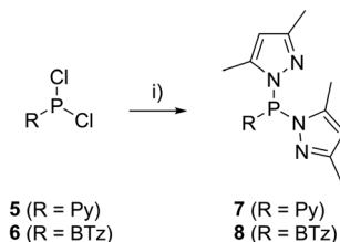
Scheme 3 Synthesis of dipyrazolylphosphanes 7 and 8; R = Py; (i) 2 eq. pyrSiMe 3 , neat, –2 Me 3 SiCl; R = BTz; (i) 2 eq. pyrSiMe 3 , Et 2 O, –2 Me 3 SiCl.
