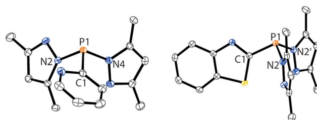
Fig. 1 Molecular structures of 7 (left) and 8 (right) (hydrogen atoms are omitted for clarity and thermal ellipsoids are displayed at 50% probability). Selected bond lengths (Å) and angles (°): (7) P1–C1 1.827(1), P1–N4 1.721(1), P1–N2 1.724(1), C1–P1–N4 101.28(5), N4–P1–N2 103.26(5), N2–P1–C1 100.18(5); (8) P1–C1 1.828(2), P1–N2 1.719(1), C1–P1–N2 101.26(5), N2–P1–N2' 103.84(7).
