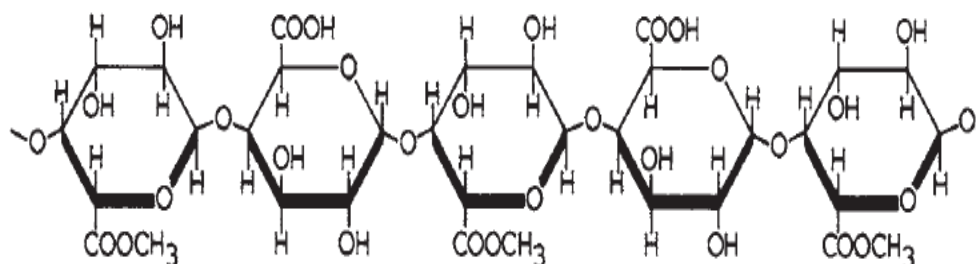
Figure 1. Pectin backbone structure, adapted from [49].
