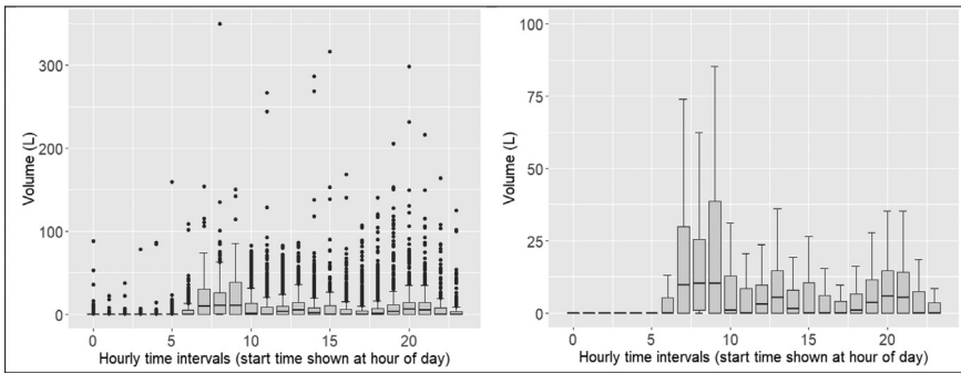
Fig. 1. Average daily hydrographs (volume in L / hourly interval) covering the entire data acquisition period of house H_{10} : with the validated complete dataset (left), after removal of the statistically outlying values (right).
