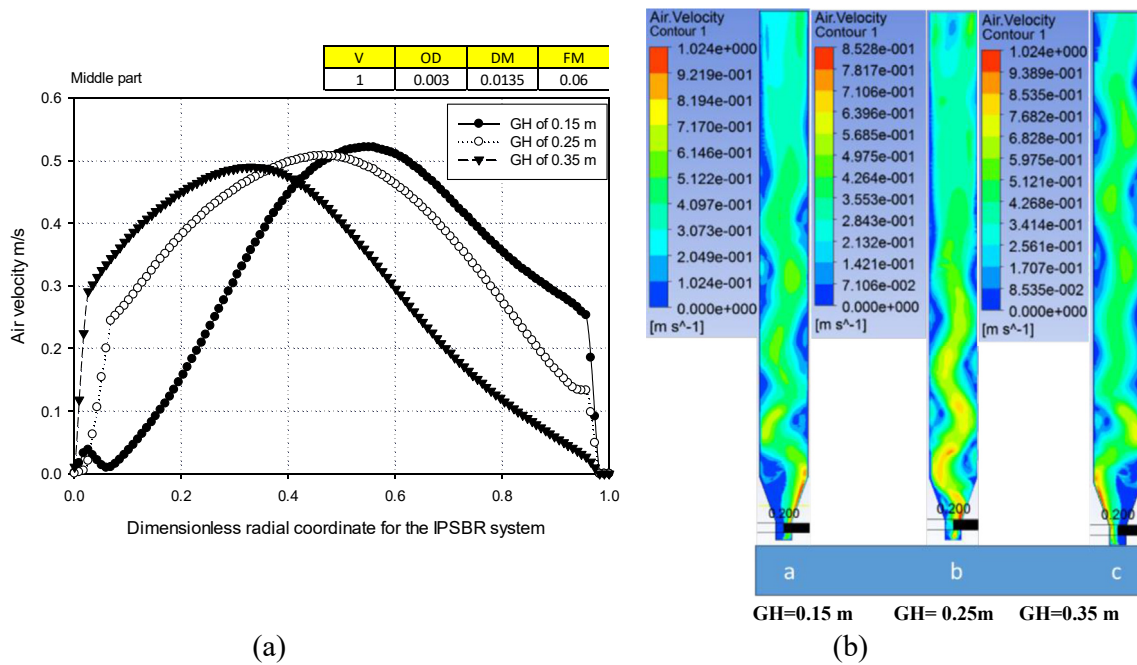
Figure 6. (a) Effect of gas head on the horizontal profile of the time-averaged gas velocity at constant feed gas velocity of 1 m/s, orifice diameter of 0.003 m, mixing particles diameter of 0.0135 m and mixing particles loading of 0.06 kg at the middle region and (b) Eulerian model contours over the three regions for the effect of gas head on the air velocity distribution at the same fixed conditions.
