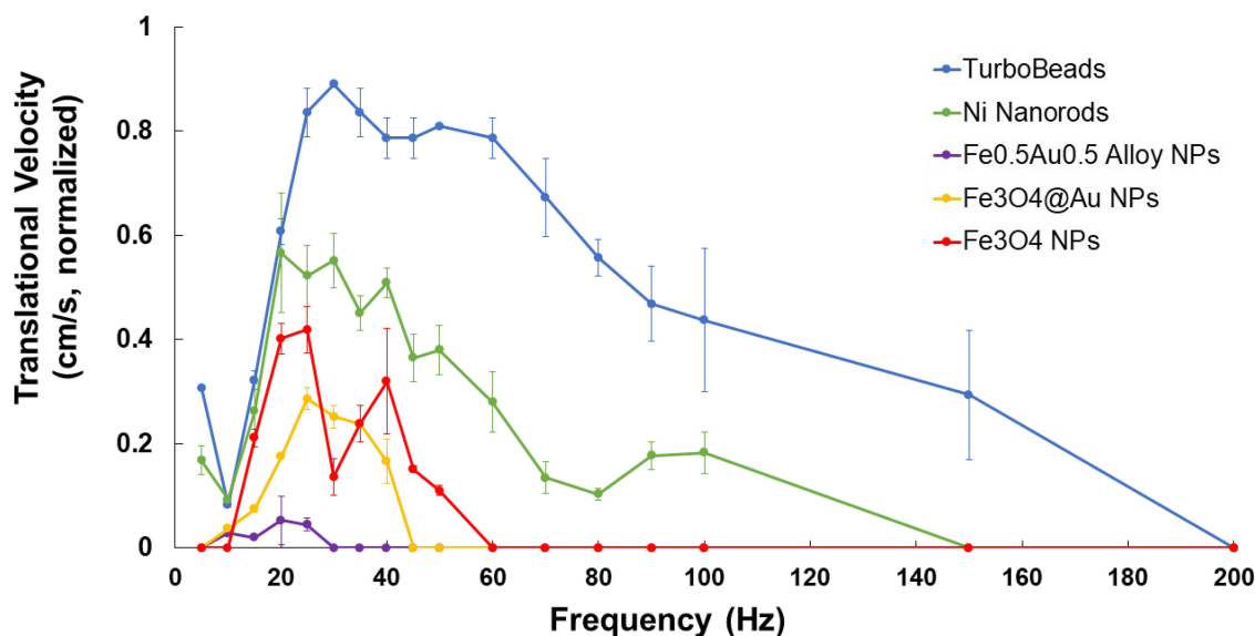
Figure 5 Translational velocities for the five MNPs, plotted as a function of magnetic field frequency (Hz). All MNPs experienced a critical frequency between 20 Hz and 30 Hz, after which point velocity decreased with further increases in rotational frequency. NiNRs and TurboBeads continued to travel down the tray lanes at frequencies up to 150 Hz and 200 Hz, respectively. The iron based MNPs tested here did not have appreciable velocities above 60 Hz. These data indicate the tuneable nature of the MMS, and the variation in MNP responses.
