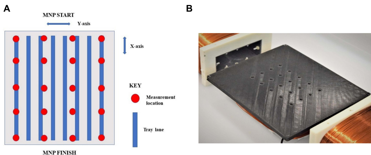
Figure 2 (A) Schematic for the magnetic field measurements. (B) Photograph of 3D-printed holder for the gauss meter probe.
