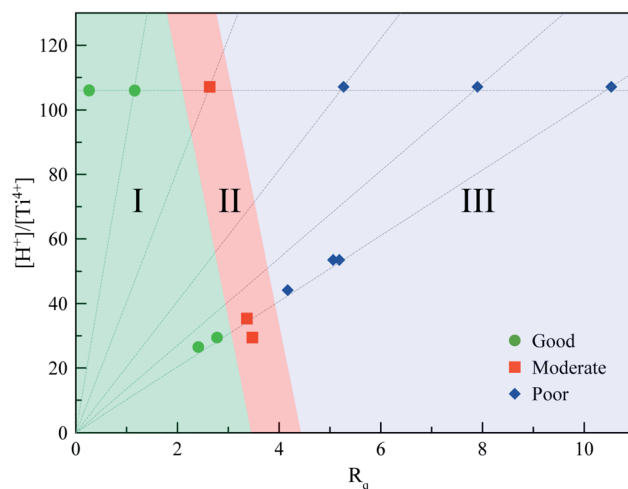
Fig. 4 Nanorod film quality classification versus R_q . The ratio R_q defined as [\text{H}^+]\text{M}_{\text{cat}}/[\text{TTIP}]V_{\text{sol}} where [\text{H}^+] and [\text{TTIP}] are the initial \text{H}^+ and TTIP concentrations ( \text{mol L}^{-1} ), while M_{\text{cat}} and V_{\text{sol}} are the mass of porous particles and the total solution volume employed in the HTVs.
