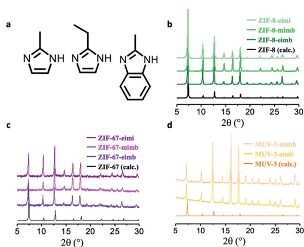
Fig. 2 (a) ZIF-8 , ZIF-67 and MUV-3 are constructed by 2-methylimidazole (mi), which is increased in size by bulkier ligands 2-ethylimidazole (ei) and 2-methylbenzimidazole (mb). (b–d) X-ray powder diffractograms of ZIF-mimib , ZIF-eimib and ZIF-eimi (b, c and d for the different metallic centres, Zn(II), Co(II) and Fe(II), respectively), showing the isoreticularity between them.
