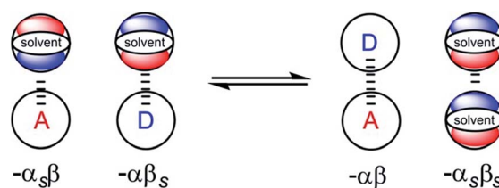
Fig. 1 Schematic representation of the electrostatic solvent competition model. The free energy of interaction between acceptor (A) and donor (D) solutes can be estimated from the H-bond parameters of the solutes ( \alpha , \beta ) and of the solvent ( \alpha_s , \beta_s ) according to eqn (1).
