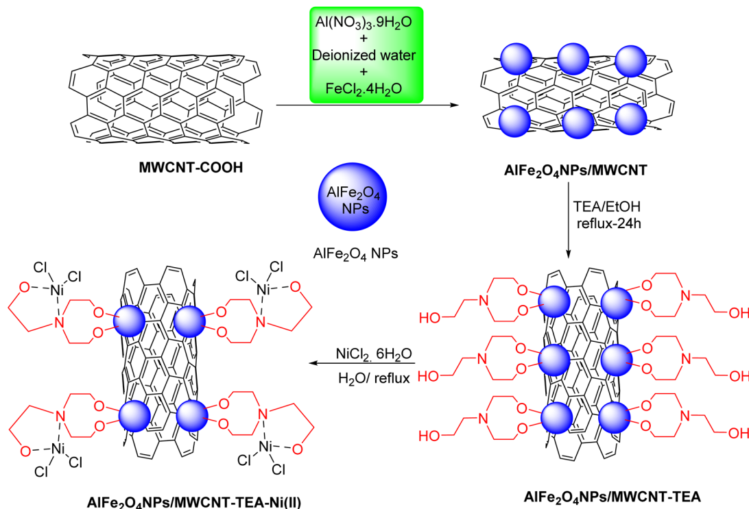
Scheme 2 Procedure for the preparation of AlFe 2 O 4 -MWCNT-TEA-Ni(II).
