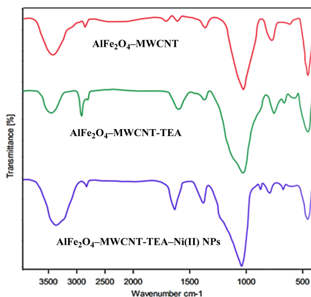
Fig. 2 FT-IR spectra of AlFe 2 O 4 @MWCNT, AlFe 2 O 4 @MWCNT-TEA, and AlFe 2 O 4 @MWCNT-TEA-Ni(II) nanocatalyst.
