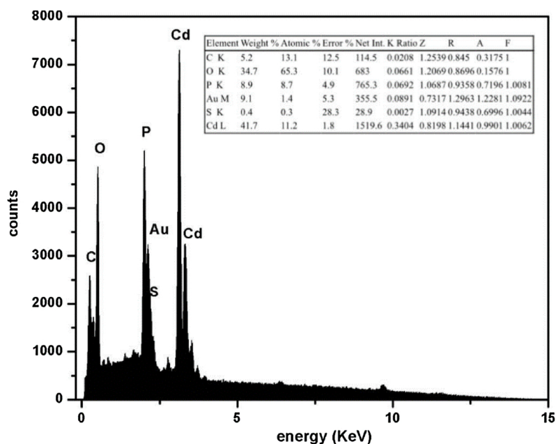
Fig. 3. EDX and elemental mapping of CdS nanoparticles. The estimated band gap value for CdS is 2.02 eV.
