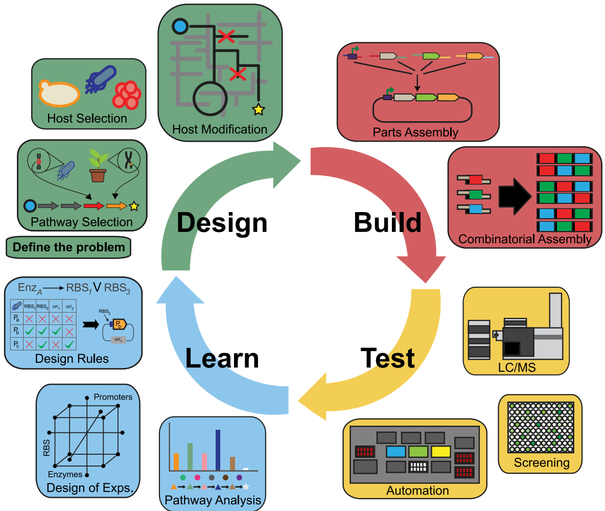
Figure 1. Typical design–build–test–learn cycle diagram from [4].
