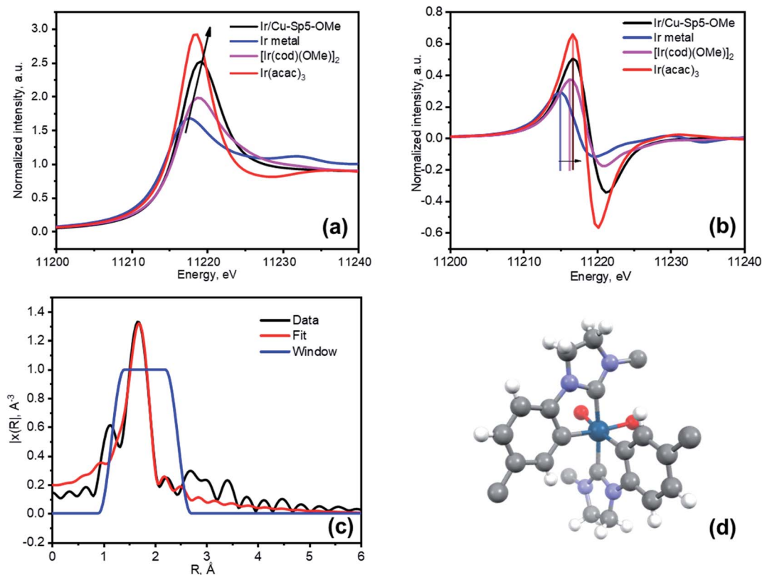
Fig. 4 (a) XANES spectra of Ir/Cu-Sp5-OMe compared to Ir metal, [\text{Ir}(\text{cod})(\text{OMe})_2] and \text{Ir}(\text{acac})_3 references, (b) First derivative of the XANES spectra from (a) and (c) Fitted EXAFS spectrum of Ir/Cu-Sp5-OMe in R -space (d) A model of iridium arrangement in Ir/Cu-Sp5-OMe. Atom colors: Ir, dark blue; C, grey; O, red; N, blue; H, white. The \text{BF}_4^- ions were omitted for clarity. While it cannot be modeled, based on the chemical species and their concentration in the reaction, it is expected that the two additional coordination sites on the Ir(III) complex, currently represented by O species, is likely to be two THF molecules.
