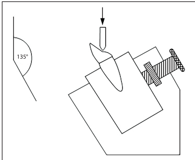
Figure 1. Schematic view of the apparatus for fracture testing with a specimen mounted in the universal testing machine at angle of 135° relation to the long axis of the posts
