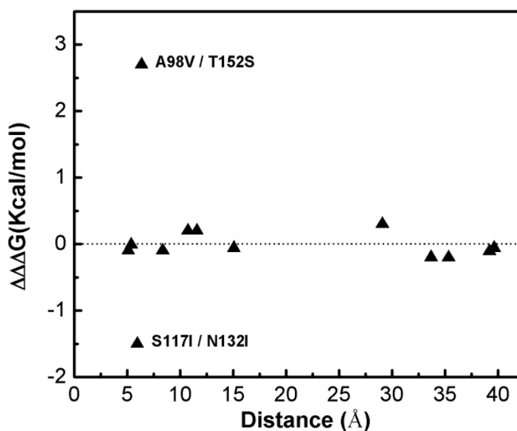
Figure 2. The dependence of the double-site mutation effects on the distances between the two corresponding single sites of the T4 phage lysozyme.
