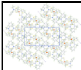
Fig. 3. A view of the supramolecular layer in the ab plane in (I) mediated by C—H...S and C—H... \pi interactions shown as orange and purple dashed lines, respectively.
