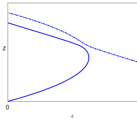
(b) Steady state solutions for c_4 < 0, c_6 < 0 .
