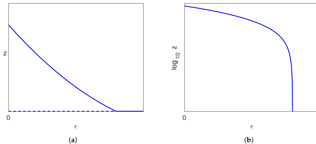
Figure 10. A typical bifurcation diagram for the Neumann/Dahari models, where solid lines indicate stable solutions and dashed lines indicate unstable solutions. Note that the vertical scale is either (a) z or (b) \log_{10} z .
