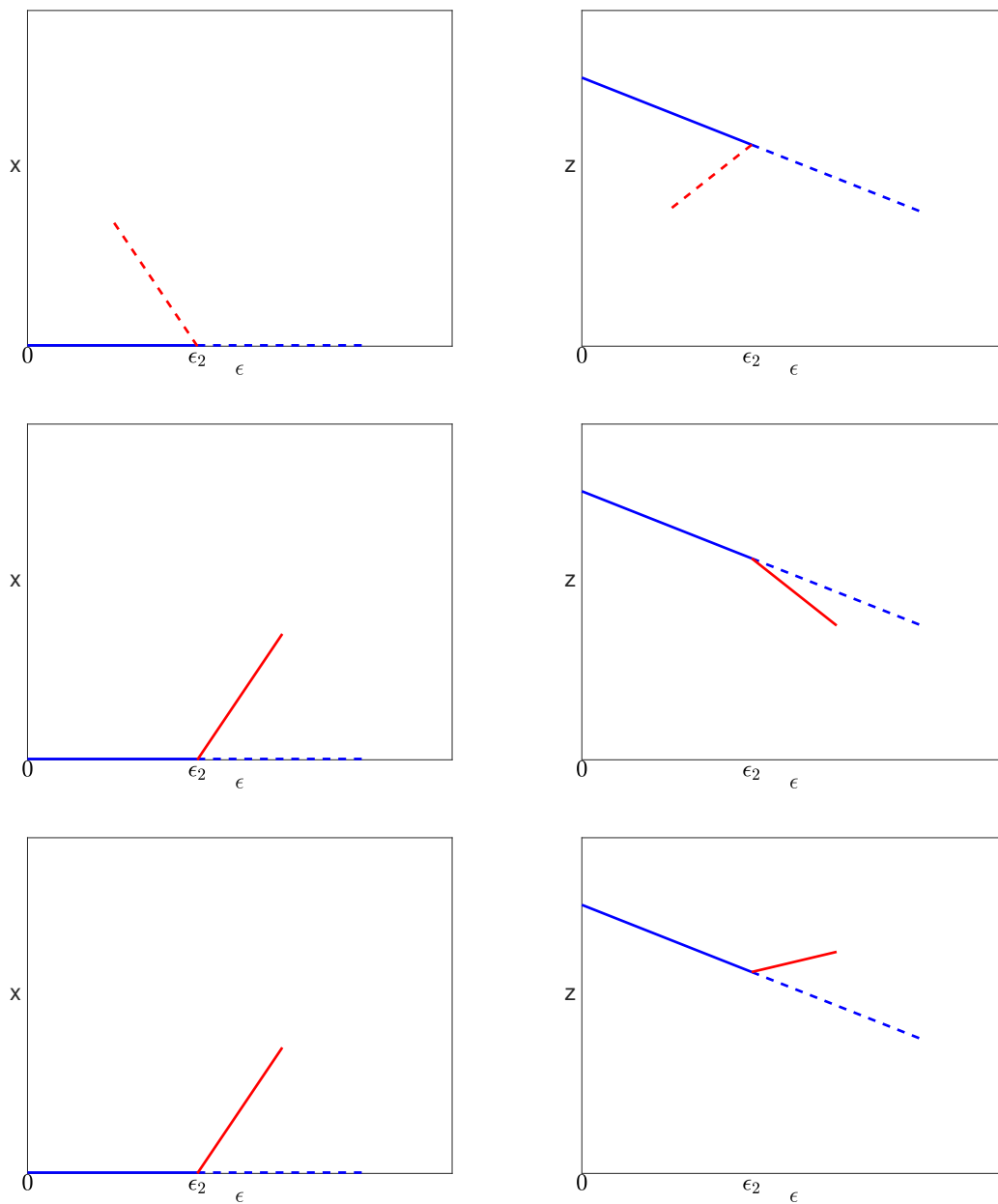
Figure 4. Solutions near the bifurcation involving the infected (red) and pure infection (blue) branches. Solid lines indicate stable solutions, while dashed lines represent unstable solutions. Top: c_4 > 0 . Middle: c_4 < 0, c_6 < 0 . Bottom: c_4 < 0, c_6 > 0 .
