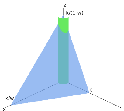
Figure 3. The invariant region in the positive octant bounded by the cylinder \mathcal{C} (see Theorem 1) and the plane (34).
