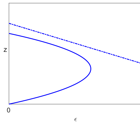
Figure 8. The steady state solutions when (73) holds and S > 0 . The dashed-dotted line consists of invalid solutions as x < 0 .
