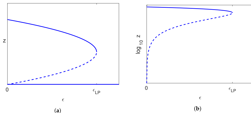
Figure 9. The bifurcation diagram, where solid lines indicate stable solutions and dashed lines indicate unstable solutions. Note that the vertical scale is either (a) z or (b) \log_{10} z .
