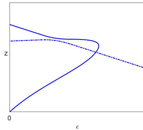
(c) Steady state solutions for c_4 < 0, c_6 > 0 .
