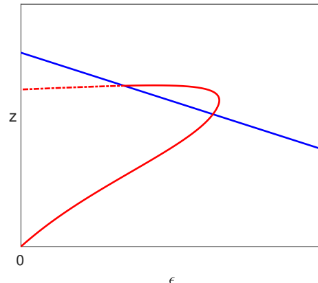
(c) The infected branch for c_4 < 0, c_6 > 0 .
