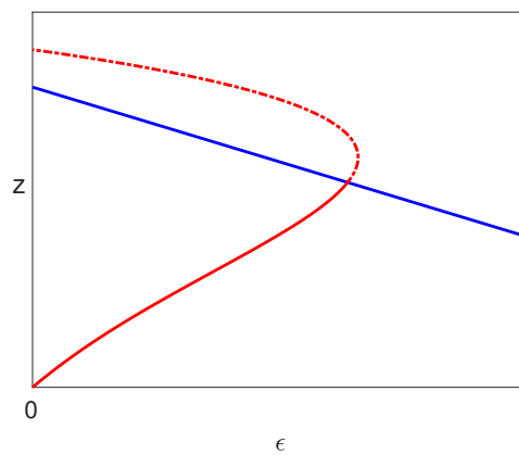
(a) The infected branch for c_4 > 0 .
