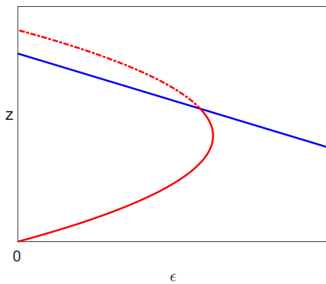
(b) The infected branch for c_4 < 0, c_6 < 0 .
