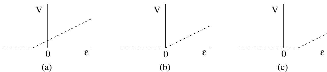
Figure 2. The bifurcation from the uninfected steady state. The bifurcation point occurs for (a) \epsilon < 0 , (b) \epsilon = 0 , (c) \epsilon > 0 . Stable steady states are indicated by solid lines and unstable steady states by dashed lines.
