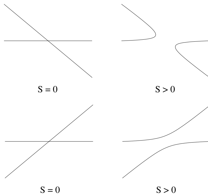
Figure 6. Unfolding of the transcritical bifurcation given by (72) in the (\epsilon, x) plane for c_4 > 0 (top) and c_4 < 0 (bottom).
