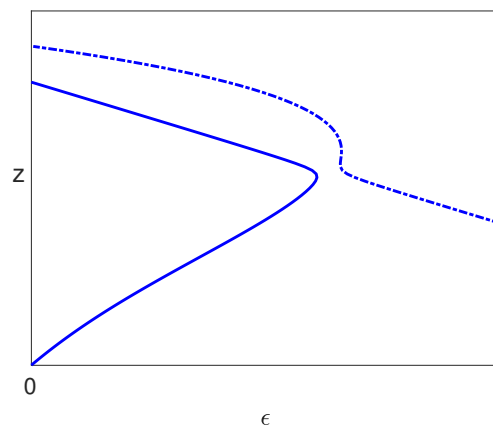
(a) Steady state solutions for c_4 > 0 .
