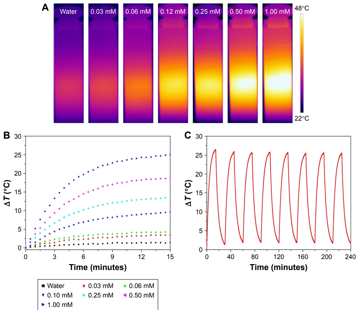
Figure 3 Photothermal performance of the GA-Fe@BSA NPs. Notes: (A) NIR thermal images and (B) temperature variations of GA-Fe@BSA NPs at increasing concentrations, after laser ablation in the same conditions. (C) Photostability tests for water dispersion of GA-Fe@BSA NPs after eight laser on/off cycles. Abbreviations: NIR, near-infrared; GA, gallic acid; NPs, nanoparticles.
