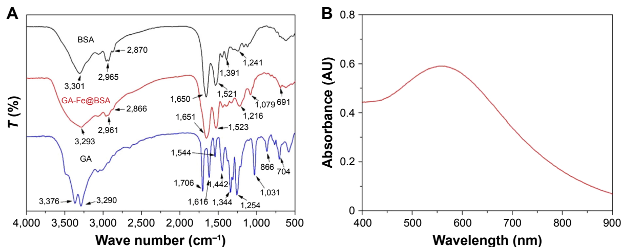
Figure 2 FT-IR (A) and UV-visible NIR absorption spectra (B) of GA-Fe@BSA NPs. Abbreviations: FT-IR, Fourier-transform infrared; UV, ultraviolet; NIR, near-IR; GA, gallic acid; NPs, nanoparticles.
