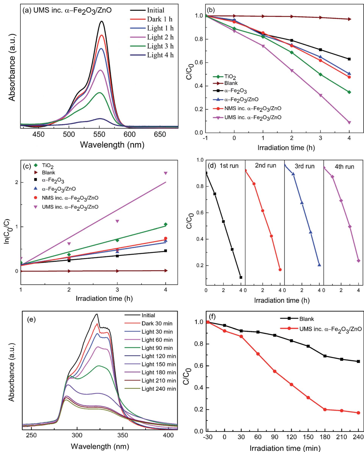
Fig. 4 (a) Time-dependent absorption spectra of RhB solution after being irradiated by solar light in the presence of ultrasonicated \text{MoS}_2 incorporated \alpha\text{-Fe}_2\text{O}_3/\text{ZnO} nanocomposite; (b) degradation of RhB as a function of the irradiation time for titania, blank sample, \alpha\text{-Fe}_2\text{O}_3 , \alpha\text{-Fe}_2\text{O}_3/\text{ZnO} , non-ultrasonicated \text{MoS}_2 incorporated \alpha\text{-Fe}_2\text{O}_3/\text{ZnO} and ultrasonicated \text{MoS}_2 incorporated \alpha\text{-Fe}_2\text{O}_3/\text{ZnO} nanomaterials; (c) pseudo-first order kinetics for RhB; (d) recyclability of ultrasonicated \text{MoS}_2 incorporated \alpha\text{-Fe}_2\text{O}_3/\text{ZnO} for 4 successive runs of photocatalytic RhB dye degradation; (e) time-dependent absorption spectra of ciprofloxacin solution after being irradiated by solar light in the presence of ultrasonicated \text{MoS}_2 incorporated \alpha\text{-Fe}_2\text{O}_3/\text{ZnO} nanocomposite; (f) degradation of ciprofloxacin as a function of irradiation time for blank sample and ultrasonicated \text{MoS}_2 incorporated \alpha\text{-Fe}_2\text{O}_3/\text{ZnO} nanocomposite.
