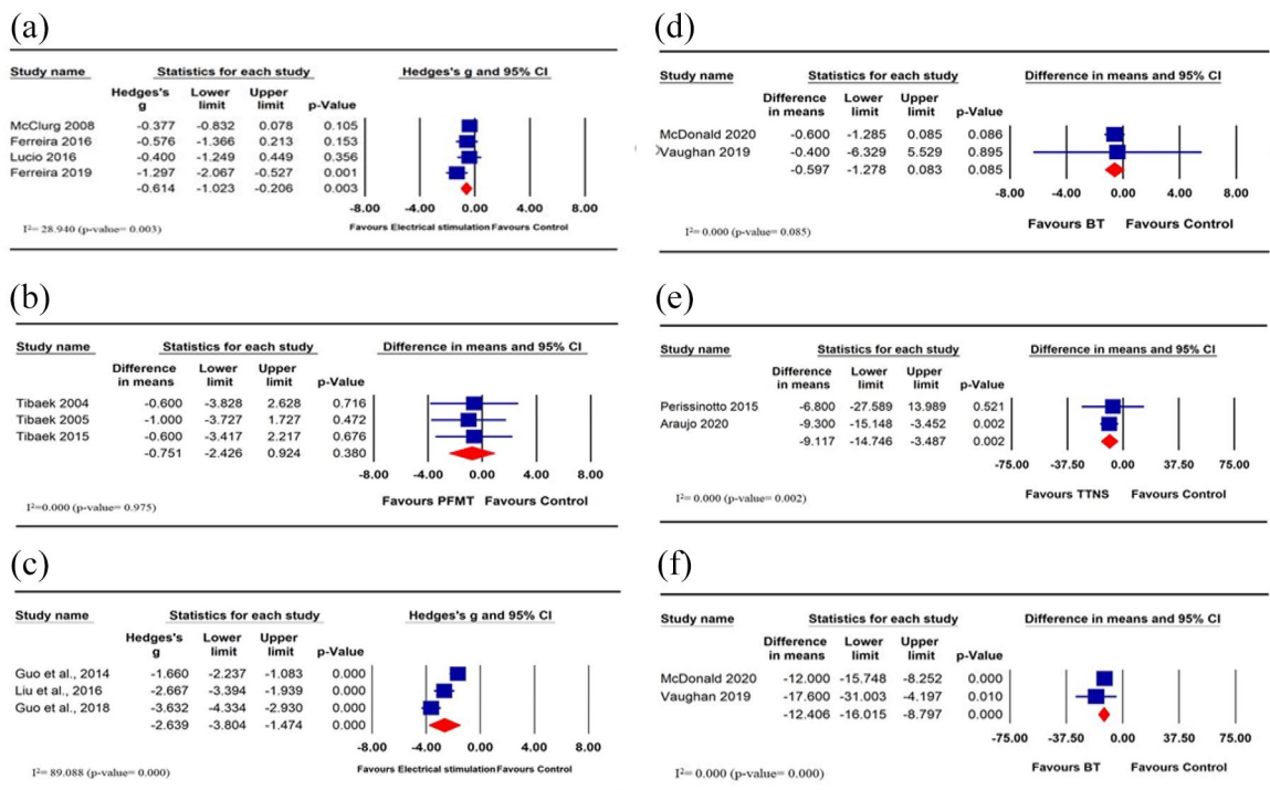
Figure 2. Forest plots. (a) Effect of electrical stimulation compared to PFMT on UUI in people with multiple sclerosis using voiding diary and OAB-V8. (b) Effect of PFMT compared to no treatment in stroke using voiding diary. (c) Effect of electrical stimulation compared to no treatment in stroke using voiding diary and OABSS. (d) Effect of BT compared with usual treatment on UUI in Parkinson's disease using voiding diary. (e) Effect of TTNS compared to no treatment in Parkinson's disease using OAB-V8. (f) Effect of BT compared to no treatment on QoL in Parkinson's disease using ICIQ-OAB.
