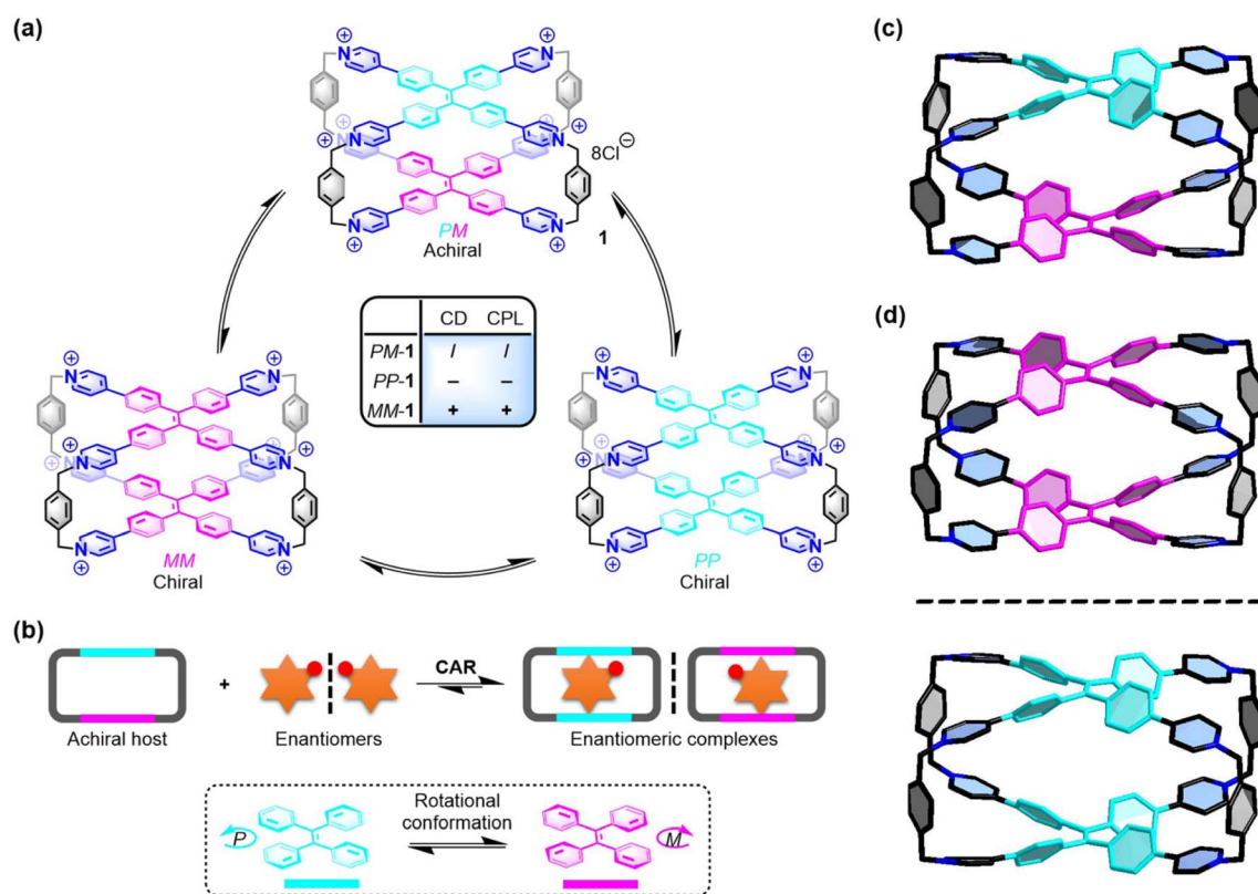
Fig. 1 (a) Three conformational isomers of 1 and their chiroptical responses. (b) Chiral adaptive recognition of 1 for enantiomers. X-ray structures of (c) PM-1 and (d) racemic MM-1 and PP-1 . Cl - counter ions and hydrogen atoms are omitted for clarity. CCDC numbers: 2100784 for PM-1 ; 2100668 for racemic MM-1 and PP-1 .†
